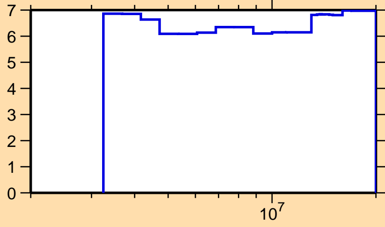
\Delta\sigma/\sigma vs. E for ^{65}\text{Co}(n,n\text{onel.})
