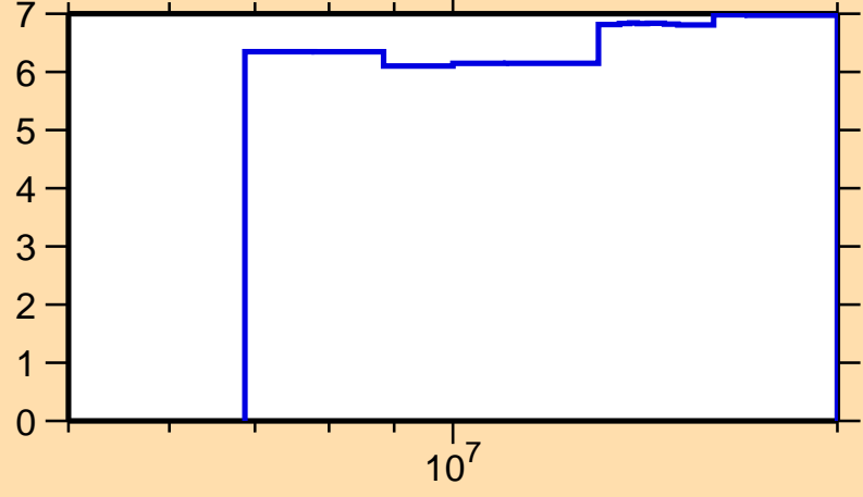
\Delta\sigma/\sigma vs. E for ^{65}\text{Co}(n,\text{nonel.})
