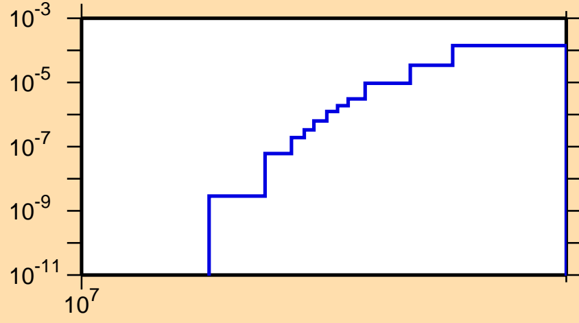
\sigma vs. E for ^{65}\text{Co}(n,t)
