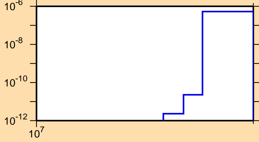
\sigma vs. E for ^{65}\text{Co}(n,nt)
