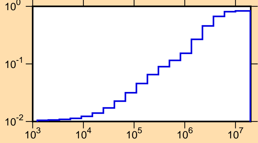
\mu vs. E for ^{65}\text{Co}(\text{mt251})
