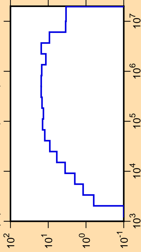
\Delta\mu/\mu vs. E for ^{65}\text{Co}(\text{mt251})
