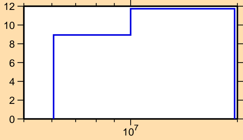
\Delta\sigma/\sigma vs. E for ^{65}\text{Co}(n,el.)
