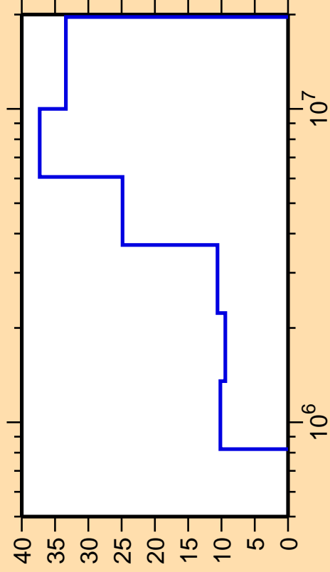
\Delta\sigma/\sigma vs. E for ^{65}\text{Co}(n,n_3)
