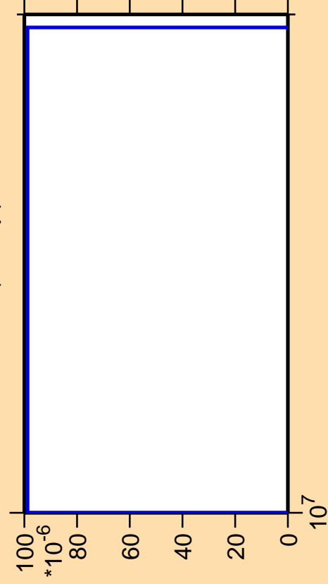
\Delta\sigma/\sigma vs. E for ^{65}\text{Co}(n,2np)
