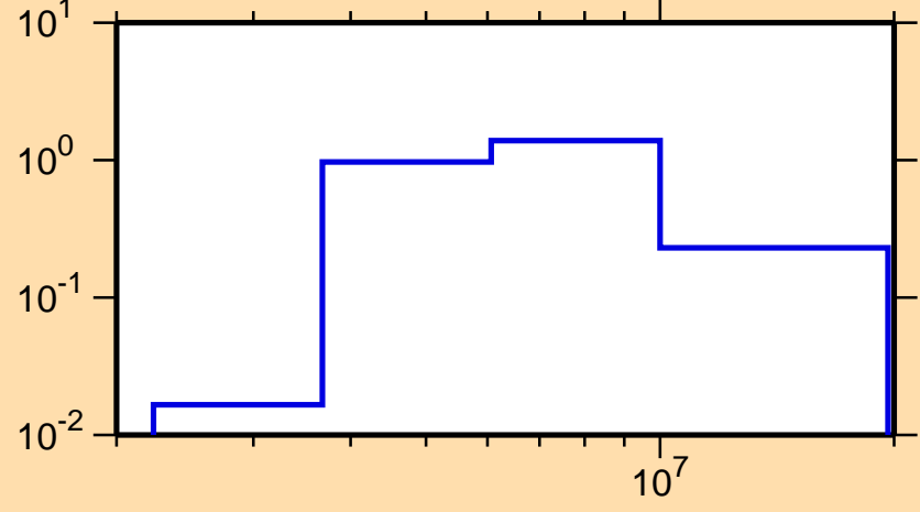
\sigma vs. E for ^{65}\text{Co}(n,n\text{cont.})
