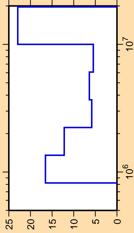
\Delta\sigma/\sigma vs. E for ^{65}\text{Co}(n,\text{inel.})
