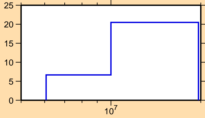
\Delta\sigma/\sigma vs. E for ^{65}\text{Co}(n,n\text{cont.})
