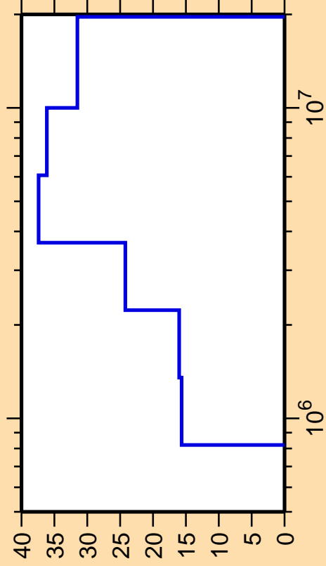
\Delta\sigma/\sigma vs. E for ^{65}\text{Co}(n,n_2)
