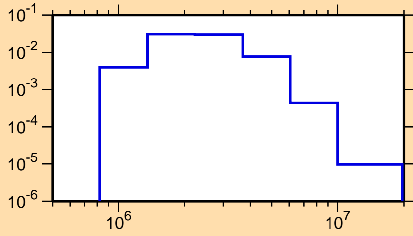
\sigma vs. E for ^{65}\text{Co}(n,n_2)
