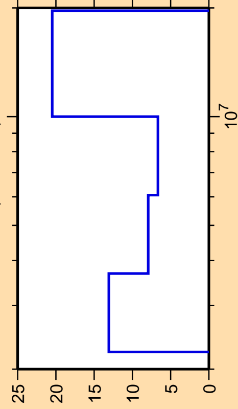
\Delta\sigma/\sigma vs. E for ^{65}\text{Co}(n,\text{ncont.})
