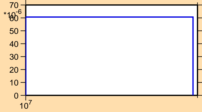
\sigma vs. E for ^{65}\text{Co}(n,np)
