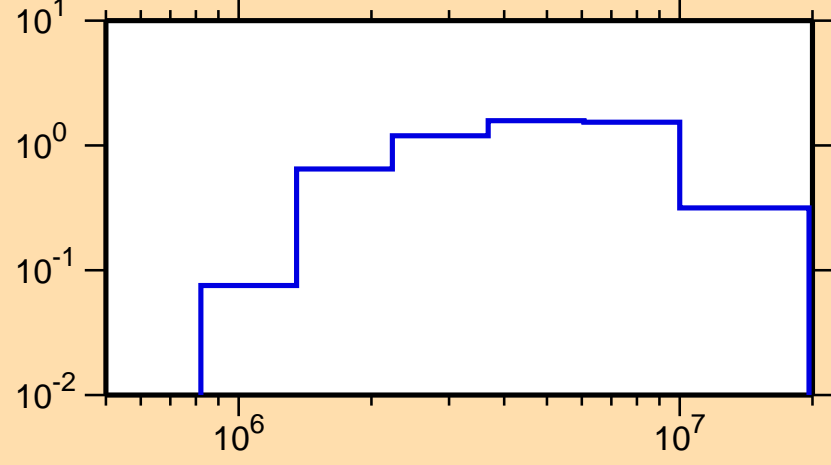
\sigma vs. E for ^{65}\text{Co}(n,\text{inel.})
