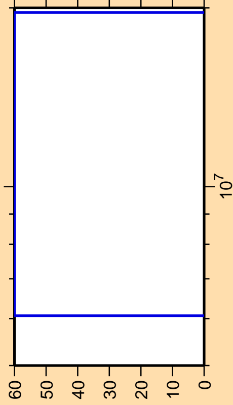
\Delta\sigma/\sigma vs. E for ^{65}\text{Co}(n,\gamma)
