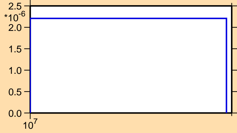
\sigma vs. E for ^{65}\text{Co}(n,\alpha)
