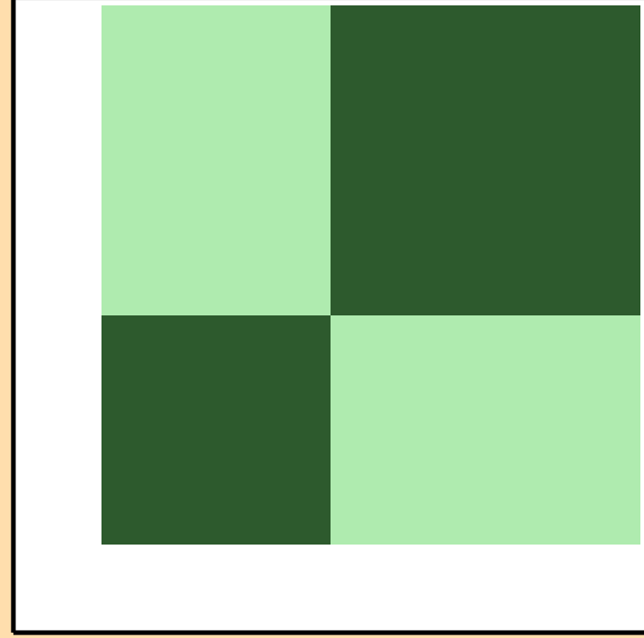
\sigma vs. E for ^{65}\text{Co}(n,d)
