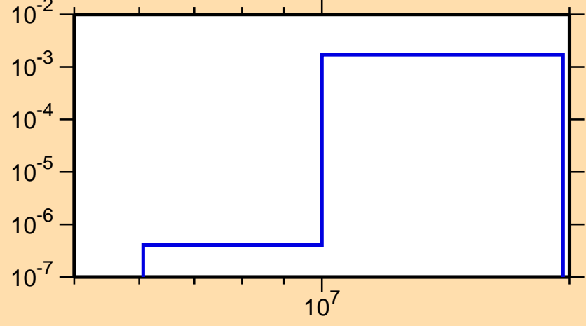
\sigma vs. E for ^{65}\text{Co}(n,p)
