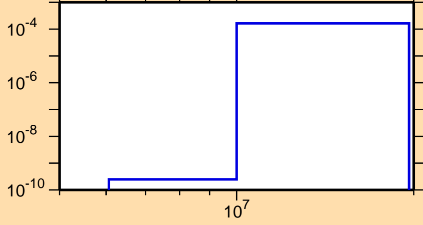
\sigma vs. E for ^{65}\text{Co}(n,\alpha)
