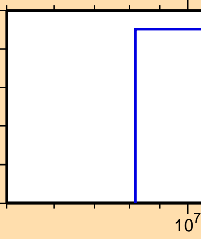
\sigma vs. E for ^{65}\text{Co}(n,2np)
