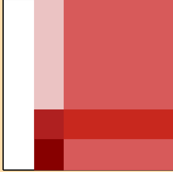
\Delta\sigma/\sigma vs. E for ^{65}\text{Co}(n,2n)
