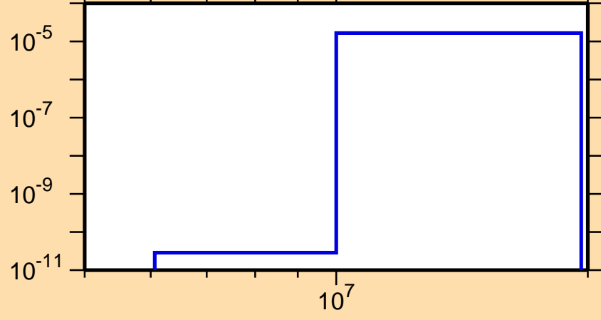
\sigma vs. E for ^{68}\text{Co}(n,\alpha)
