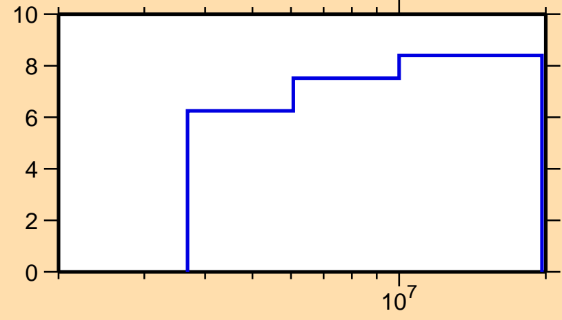
\Delta\sigma/\sigma vs. E for ^{49}\text{Cr}(n,n\text{onl.})
