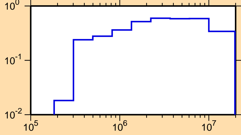
\sigma vs. E for ^{49}\text{Cr}(n,\text{inel.})
