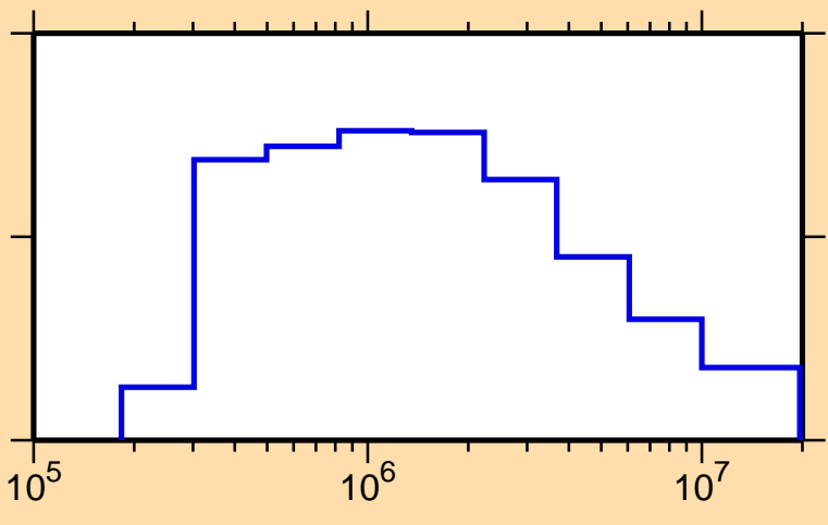
\sigma vs. E for ^{49}\text{Cr}(n,n_1)
