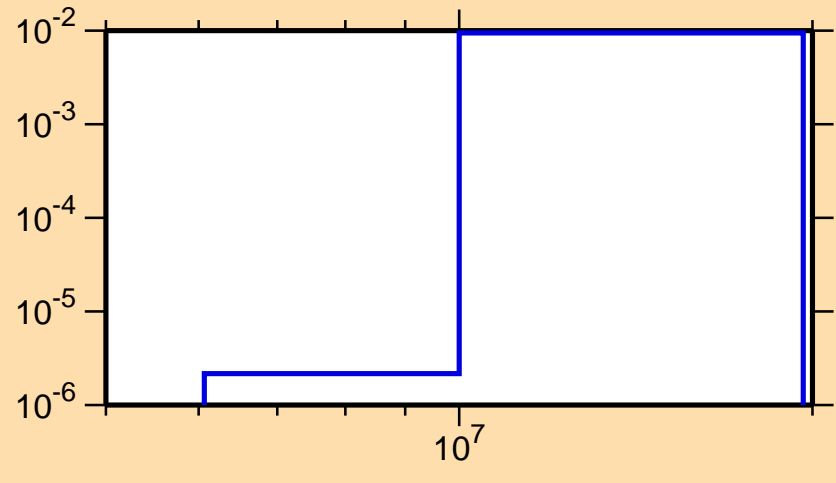
\sigma vs. E for ^{50}\text{Cr}(n,d)
