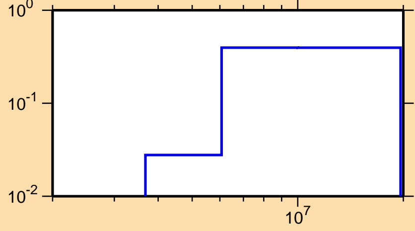
\sigma vs. E for ^{50}\text{Cr}(n,n\text{cont.})
