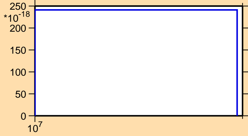
\sigma vs. E for ^{50}\text{Cr}(n,nd)
