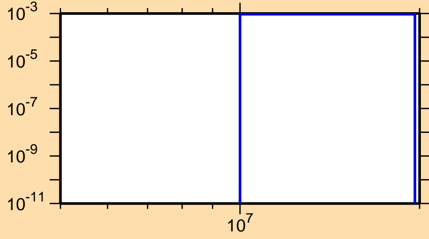
\sigma vs. E for ^{50}\text{Cr}(n,\alpha)
