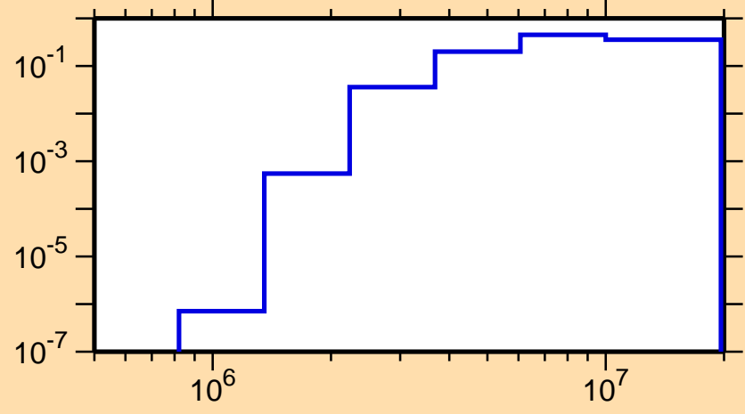
\sigma vs. E for ^{50}\text{Cr}(n,p)
