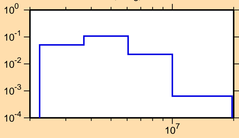
\sigma vs. E for ^{50}\text{Cr}(n,n_3)
