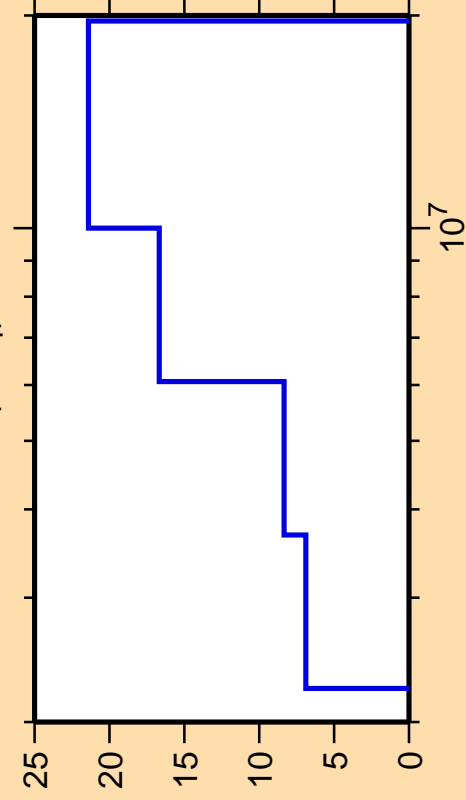
\Delta\sigma/\sigma vs. E for ^{50}\text{Cr}(n,n_4)
