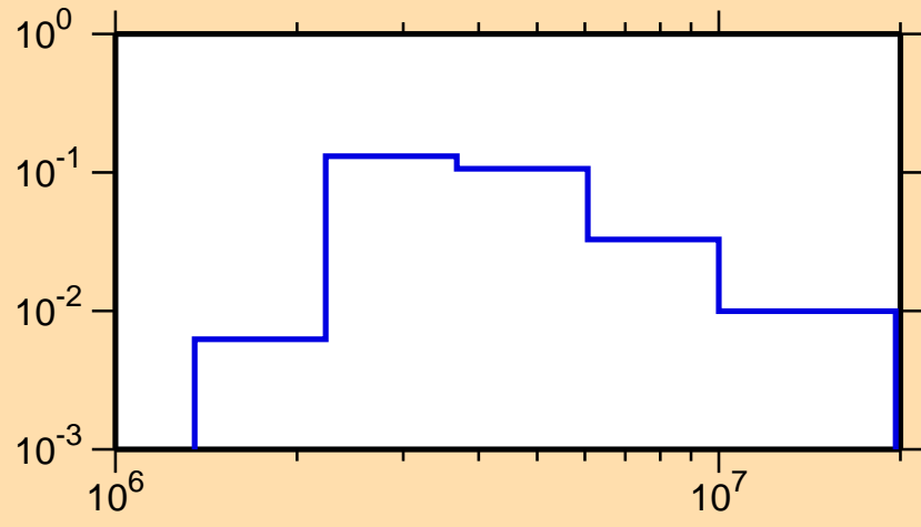
\sigma vs. E for ^{50}\text{Cr}(n,n_2)
