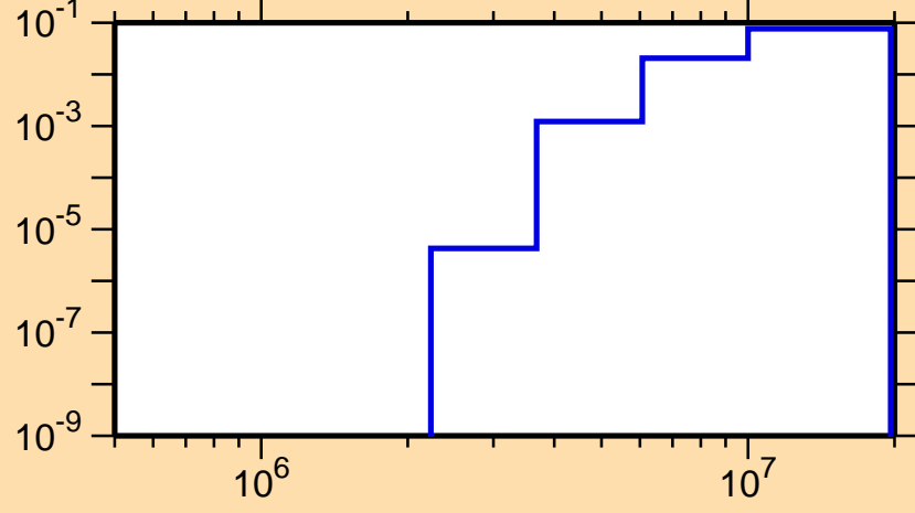
\sigma vs. E for ^{50}\text{Cr}(n,\alpha)
