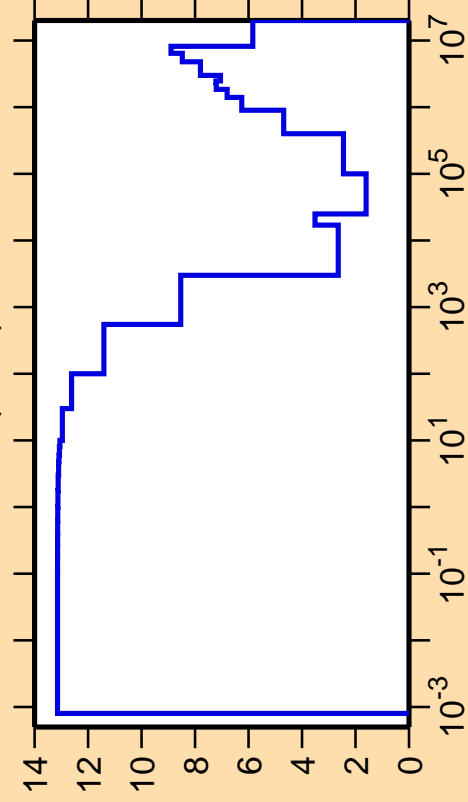
\Delta\sigma/\sigma vs. E for ^{50}\text{Cr}(n,\text{el.})
