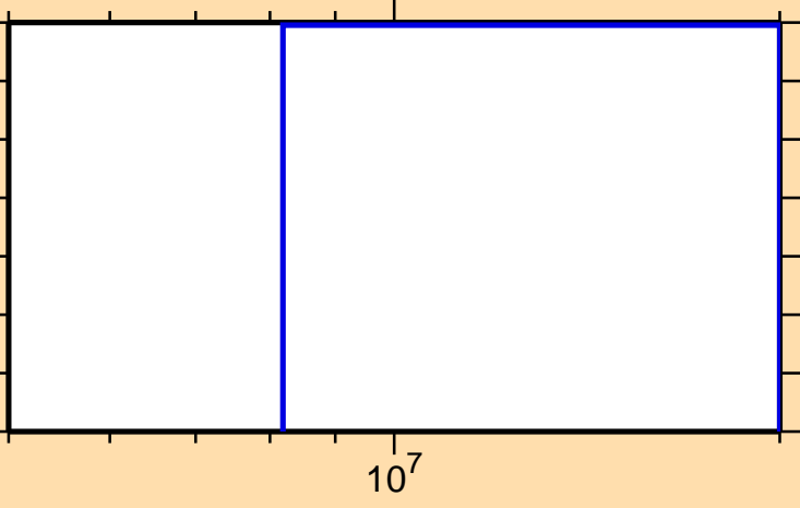
\sigma vs. E for ^{50}\text{Cr}(\text{mt } 45)
