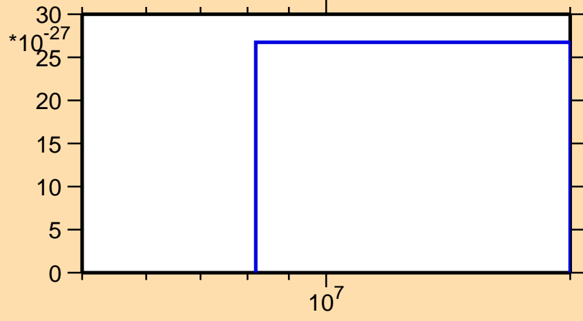
\sigma vs. E for ^{50}\text{Cr}(n,\text{pt})
