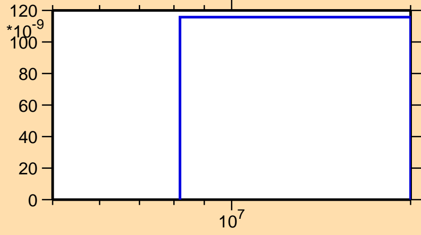
\sigma vs. E for ^{50}\text{Cr}(n,p\alpha)
