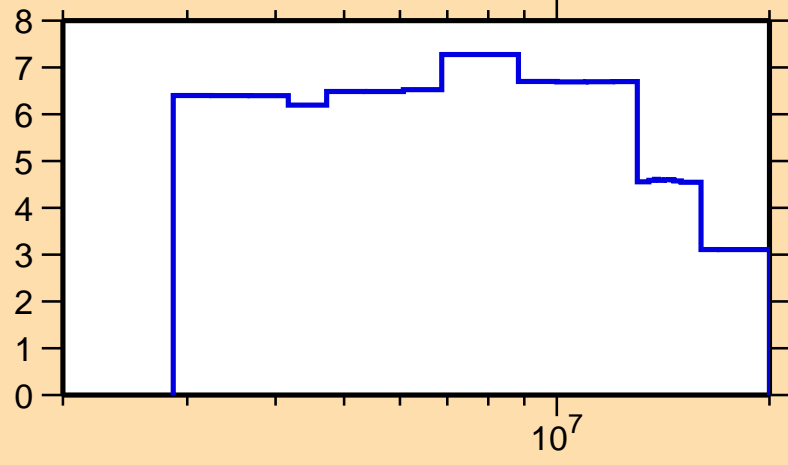
\Delta\sigma/\sigma vs. E for ^{51}\text{Cr}(n,el.)
