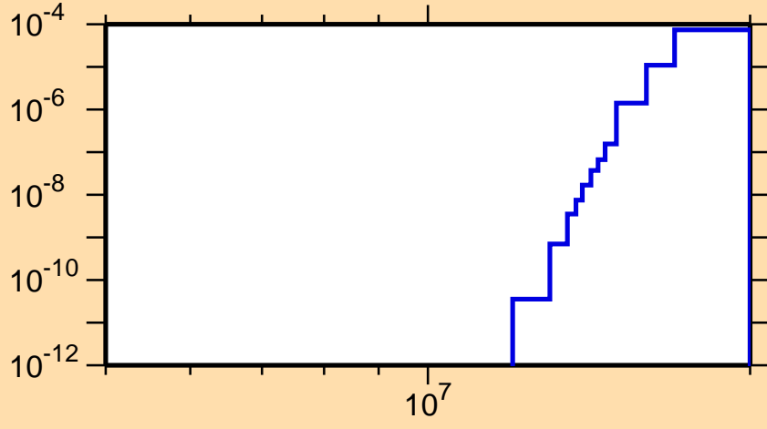
\sigma vs. E for ^{51}\text{Cr}(n,\text{He3})
