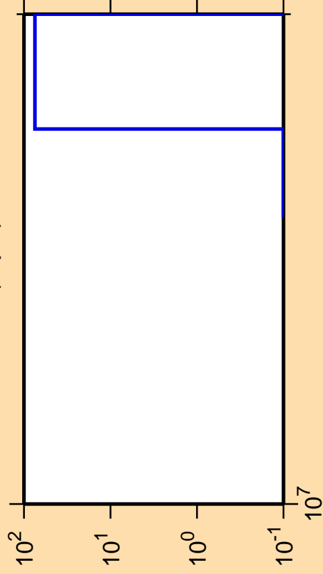
\Delta\sigma/\sigma vs. E for ^{51}\text{Cr}(n,pd)
