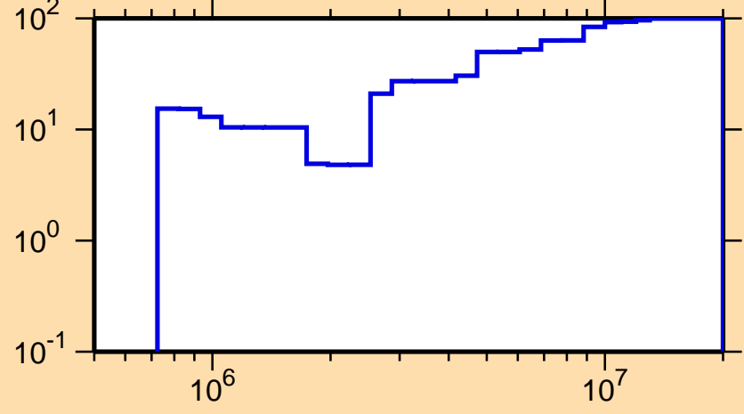
\Delta\sigma/\sigma vs. E for ^{51}\text{Cr}(n,n_1)
