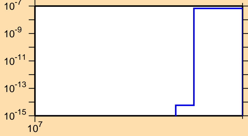
\sigma vs. E for ^{51}\text{Cr}(n,pd)
