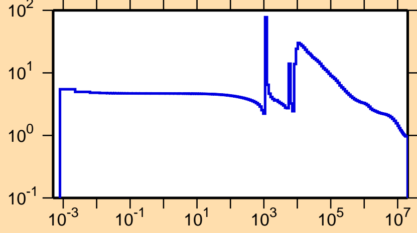
\sigma vs. E for ^{51}\text{Cr}(n,\text{el.})
