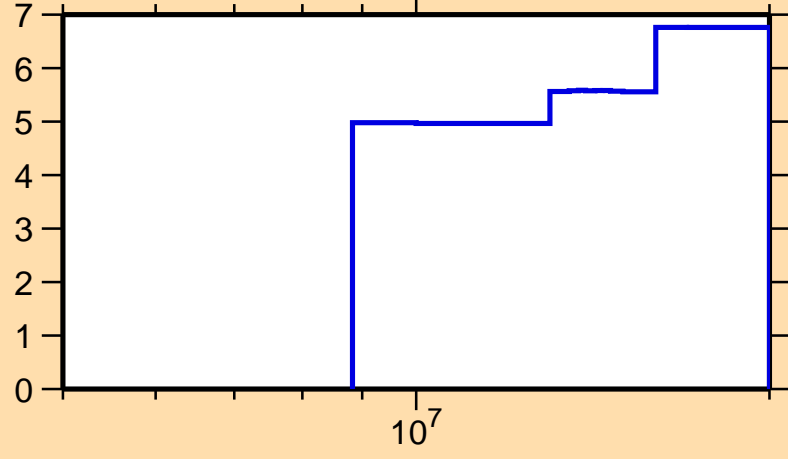
\Delta\sigma/\sigma vs. E for ^{51}\text{Cr}(n,\text{nonel.})
