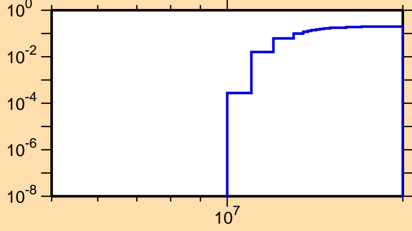
\sigma vs. E for ^{51}\text{Cr}(n,np)
