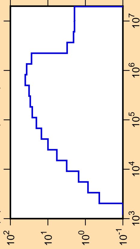
\Delta\mu/\mu vs. E for ^{51}\text{Cr}(\text{mt251})
