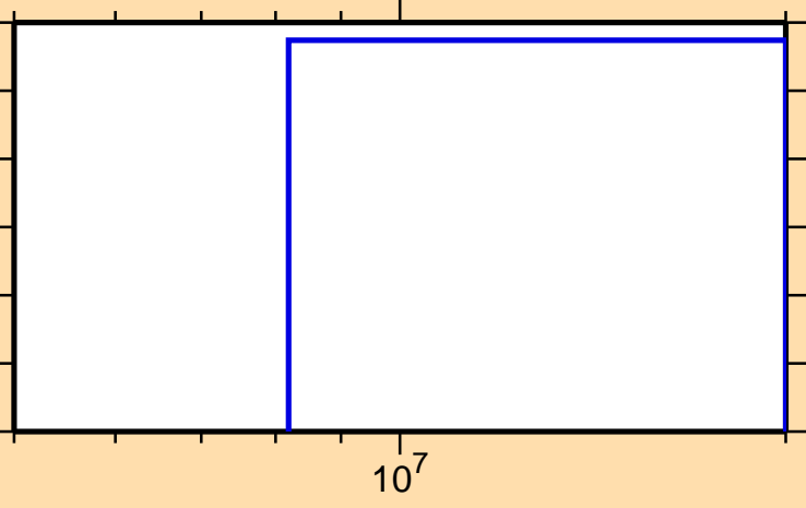
\sigma vs. E for ^{51}\text{Cr}(n,\text{nd})
