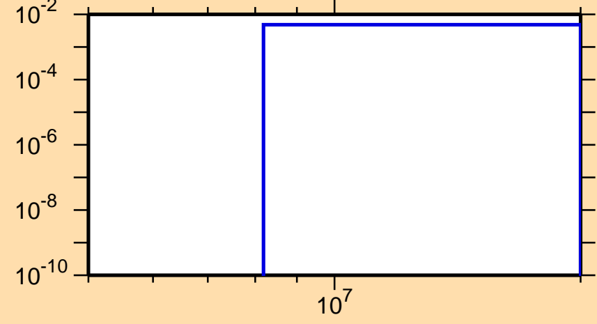
\sigma vs. E for ^{51}\text{Cr}(n,d)
