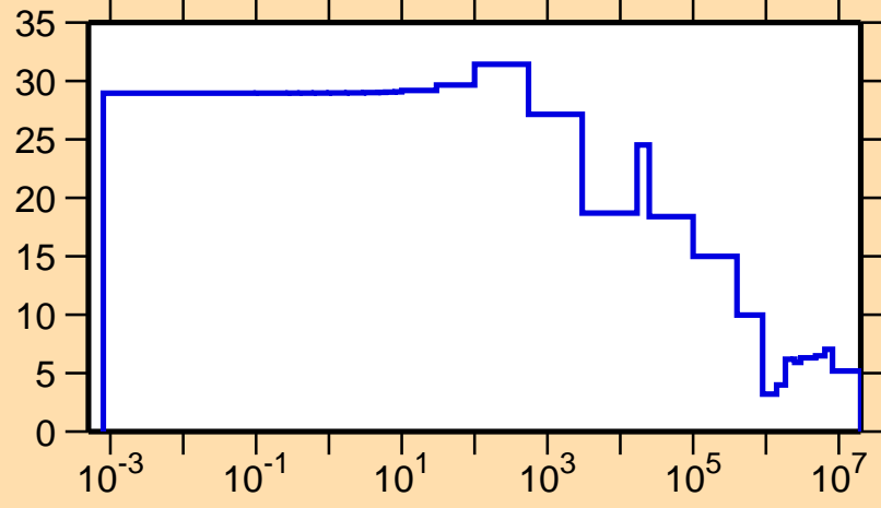
\Delta\sigma/\sigma vs. E for ^{51}\text{Cr}(n,el.)
