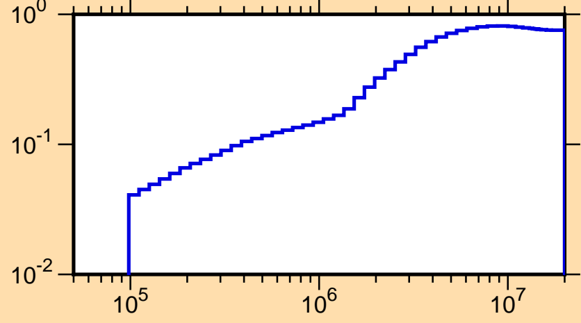
\mu vs. E for ^{52}\text{Cr}(\text{mt251})
