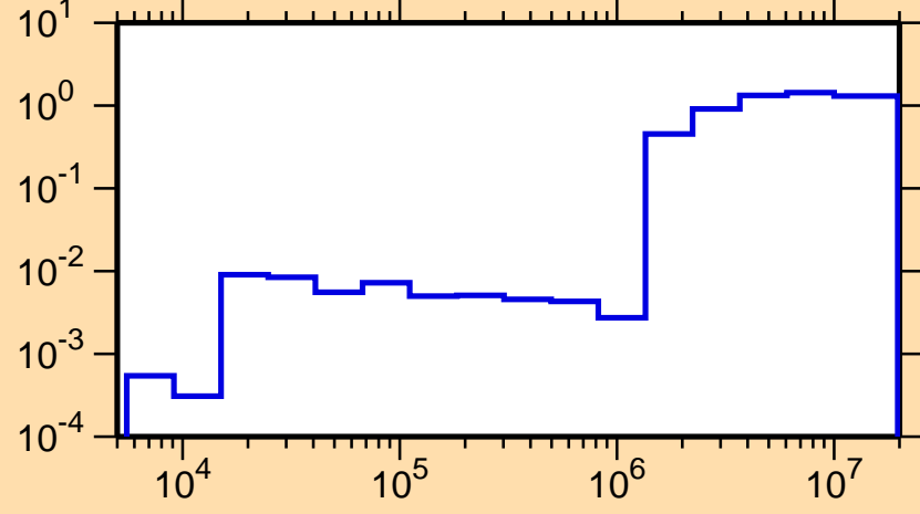
\sigma vs. E for ^{52}\text{Cr}(n,\text{nonel.})
