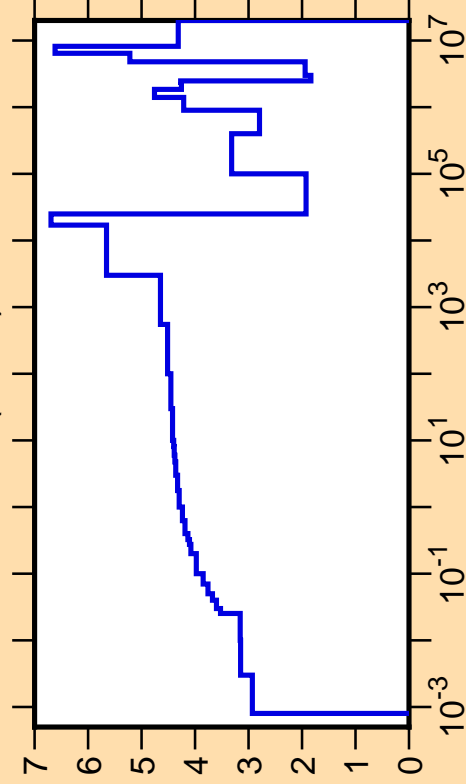
\Delta\sigma/\sigma vs. E for ^{52}\text{Cr}(n,\text{tot.})
