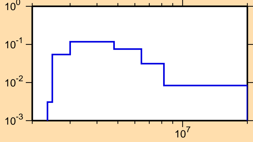
\sigma vs. E for ^{52}\text{Cr}(n,n_2)
