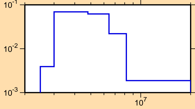
\sigma vs. E for ^{52}\text{Cr}(n,n_4)
