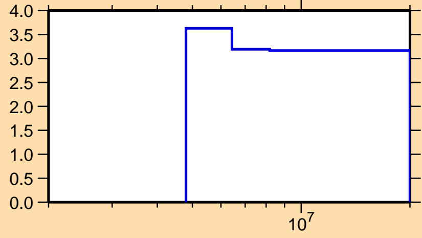
\Delta\sigma/\sigma vs. E for ^{52}\text{Cr}(n,n\text{onl.})
