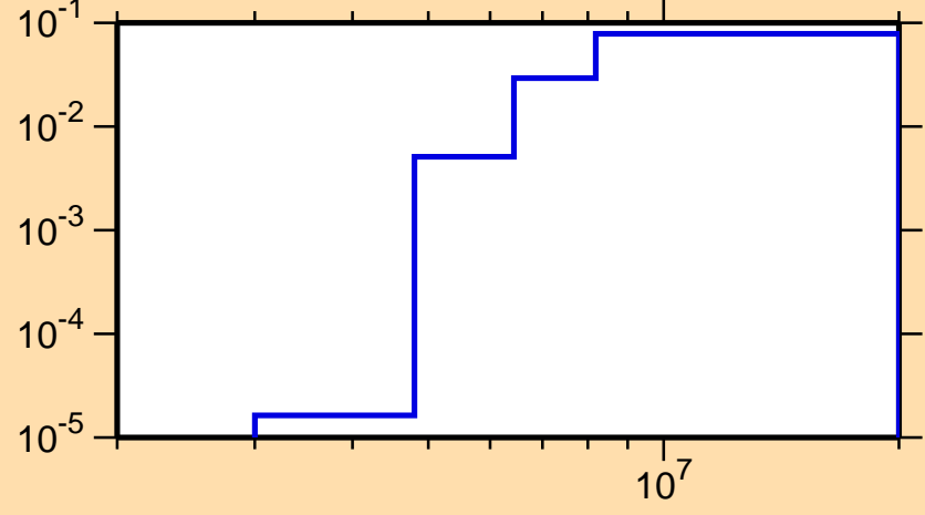
\sigma vs. E for ^{52}\text{Cr}(n,p)
