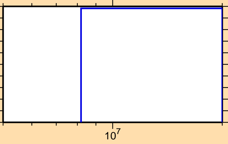
\sigma vs. E for ^{52}\text{Cr}(n,\alpha)
