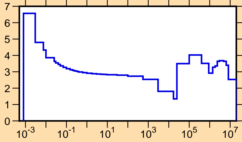
\sigma vs. E for ^{52}\text{Cr}(n,\text{tot.})
