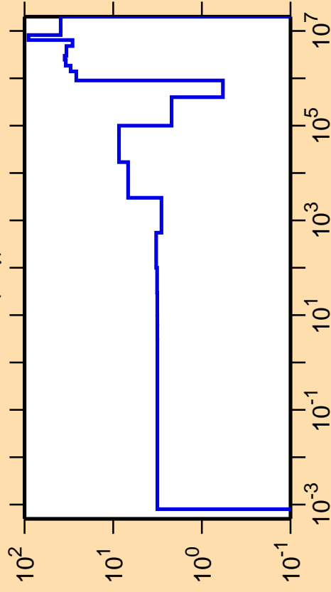
\Delta\sigma/\sigma vs. E for ^{52}\text{Cr}(n,\gamma)
