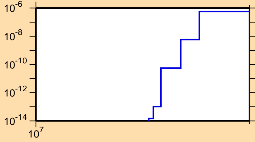
\sigma vs. E for ^{53}\text{Cr}(n,\text{He}3)
