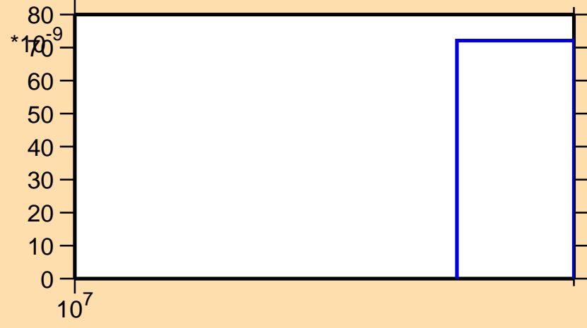
\sigma vs. E for ^{53}\text{Cr}(n,2np)
