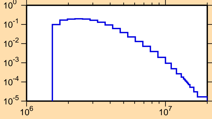
\sigma vs. E for ^{53}\text{Cr}(n,n_4)
