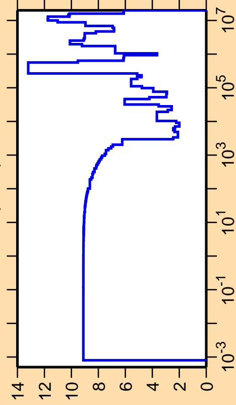
\Delta\sigma/\sigma vs. E for ^{53}\text{Cr}(n,\text{el.})
