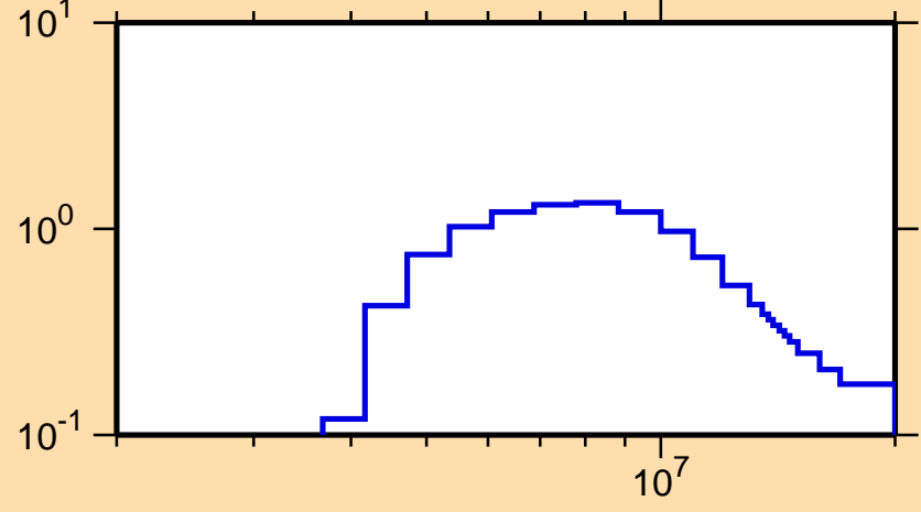
\sigma vs. E for ^{53}\text{Cr}(n,n\text{cont.})
