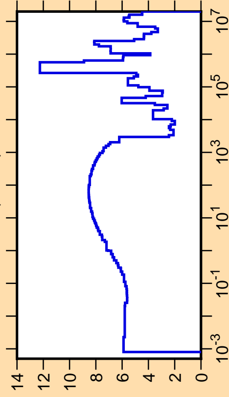
\Delta\sigma/\sigma vs. E for ^{53}\text{Cr}(n,\text{tot.})
