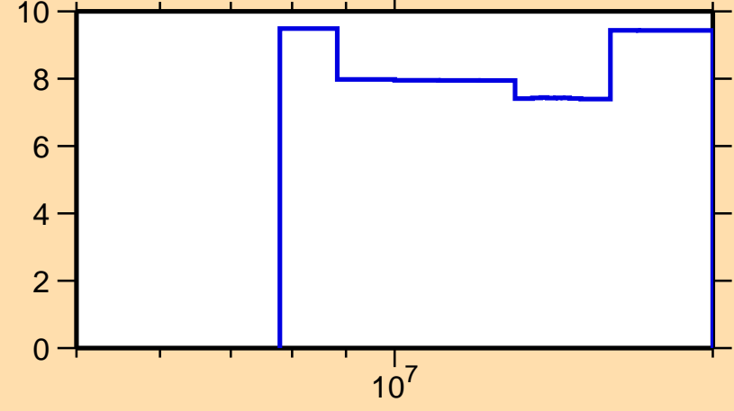
\Delta\sigma/\sigma vs. E for ^{53}\text{Cr}(n,2n)
