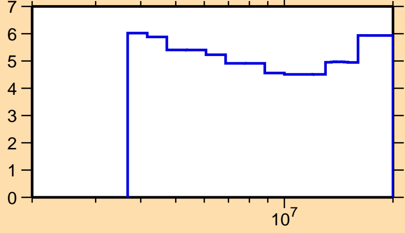
\Delta\sigma/\sigma vs. E for ^{53}\text{Cr}(n,n\text{onel.})
