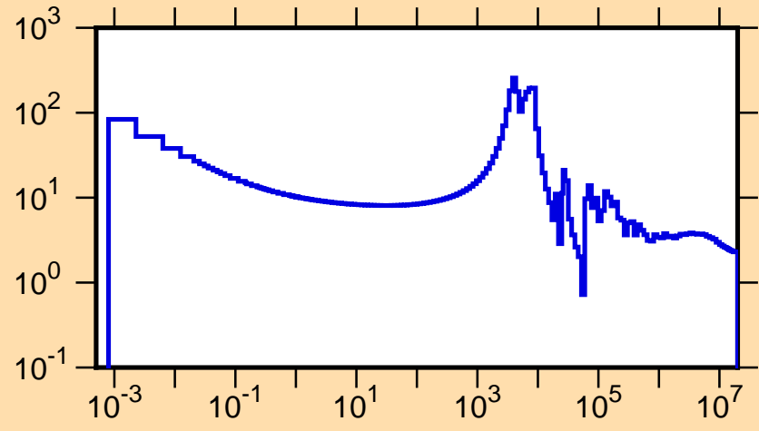
\sigma vs. E for ^{53}\text{Cr}(n,\text{tot.})
