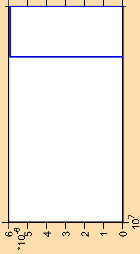
\Delta\sigma/\sigma vs. E for ^{53}\text{Cr}(n,\text{pd})
