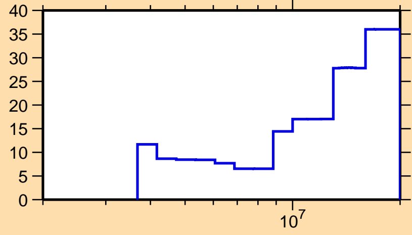
\Delta\sigma/\sigma vs. E for ^{53}\text{Cr}(n,ncont.)
