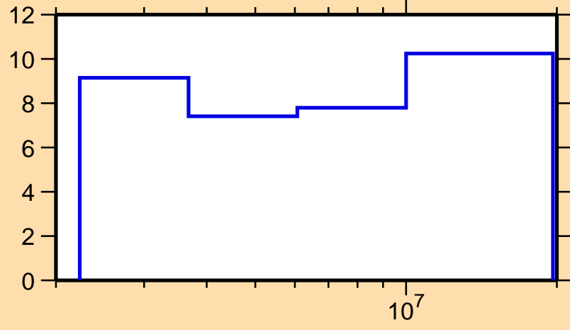
\Delta\sigma/\sigma vs. E for ^{53}\text{Cr}(n,el.)
