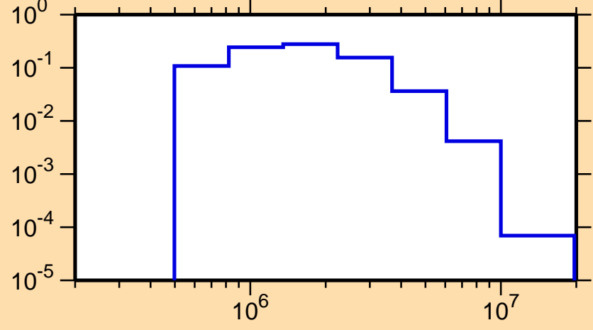
\sigma vs. E for ^{53}\text{Cr}(n,n_1)
