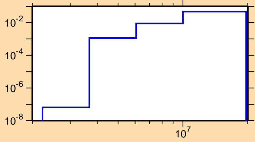
\sigma vs. E for ^{53}\text{Cr}(n,p)
