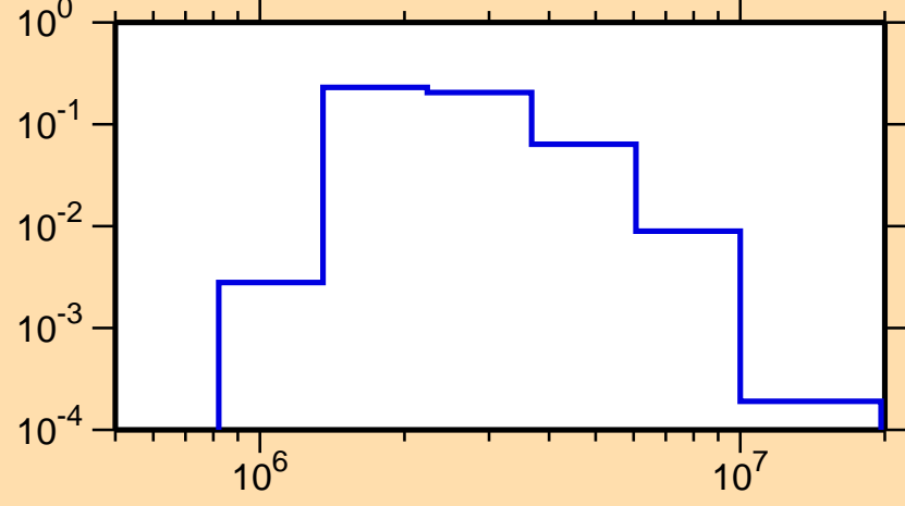
\sigma vs. E for ^{53}\text{Cr}(n,n_3)
