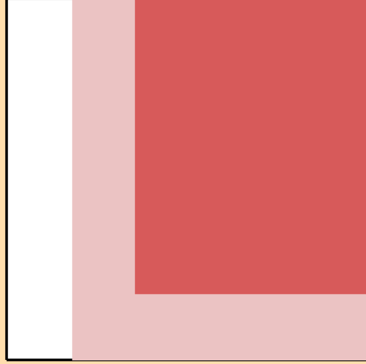
\Delta\sigma/\sigma vs. E for ^{53}\text{Cr}(n,2n)
