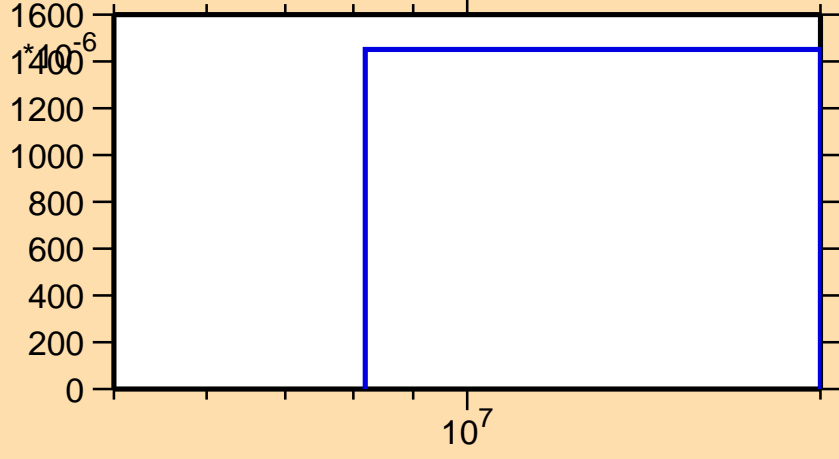
\sigma vs. E for ^{53}\text{Cr}(n,d)
