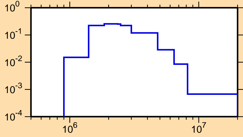
\sigma vs. E for ^{53}\text{Cr}(n,n_3)
