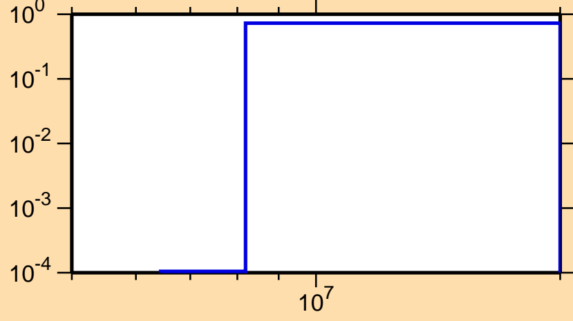
\sigma vs. E for ^{53}\text{Cr}(n,2n)
