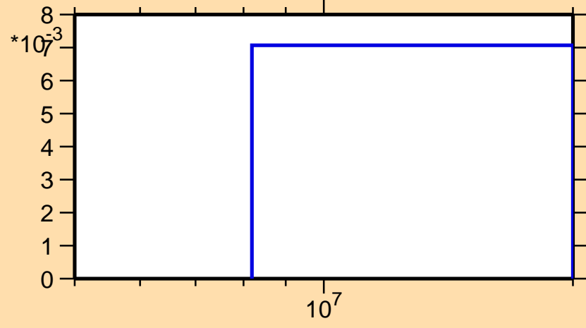
\sigma vs. E for ^{53}\text{Cr}(n,np)
