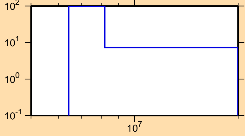
\Delta\sigma/\sigma vs. E for ^{53}\text{Cr}(n,2n)
