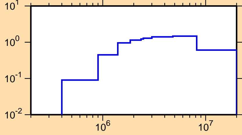
\sigma vs. E for ^{53}\text{Cr}(n,\text{inel.})
