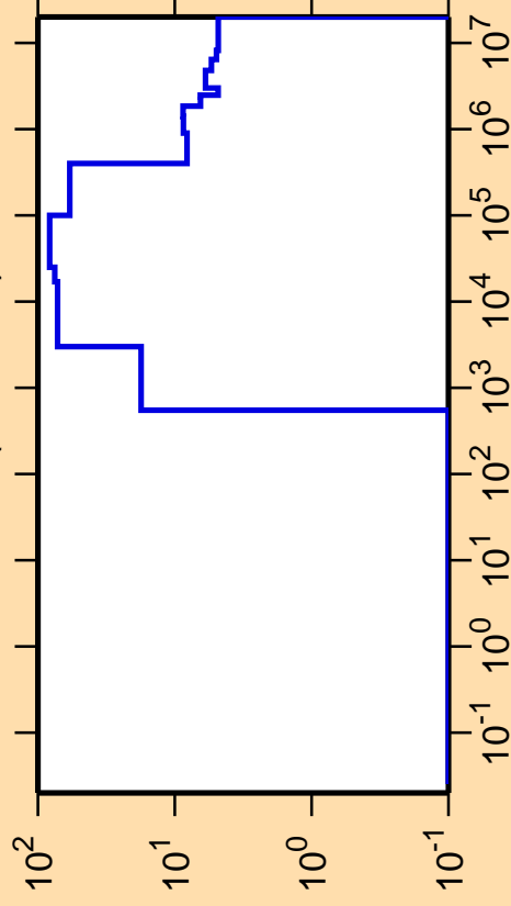
\Delta\sigma/\sigma vs. E for ^{53}\text{Cr}(n,\text{nonel.})
