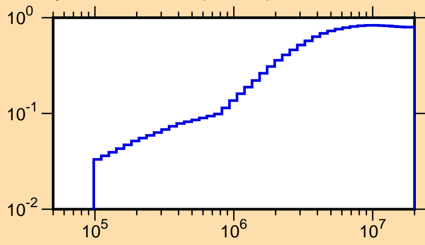
\mu vs. E for ^{54}\text{Cr}(\text{mt251})
