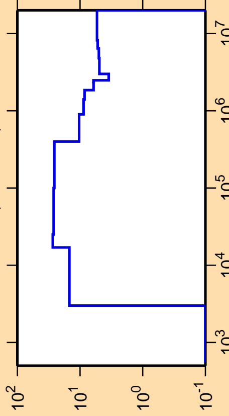
\Delta\sigma/\sigma vs. E for ^{54}\text{Cr}(n,\text{nonel.})
