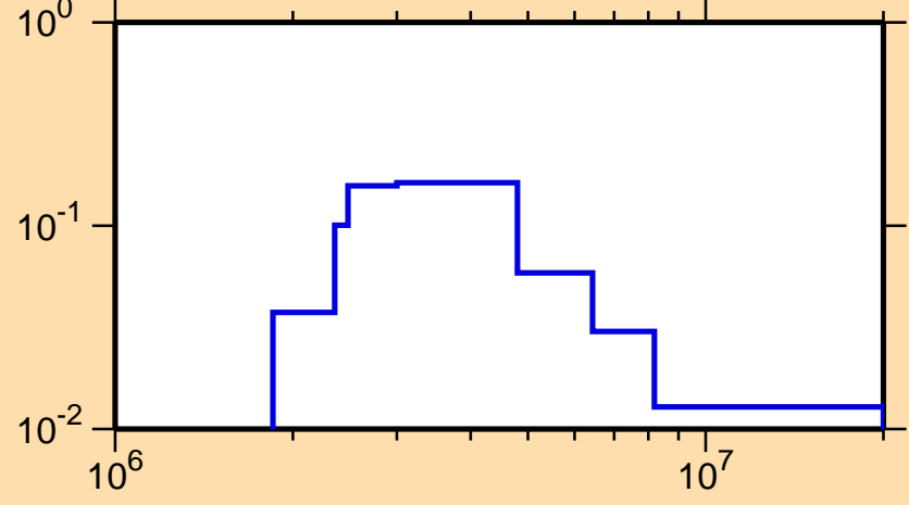
\sigma vs. E for ^{54}\text{Cr}(n,n_2)
