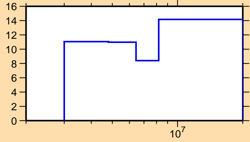
\Delta\sigma/\sigma vs. E for ^{54}\text{Cr}(n,ncont.)
