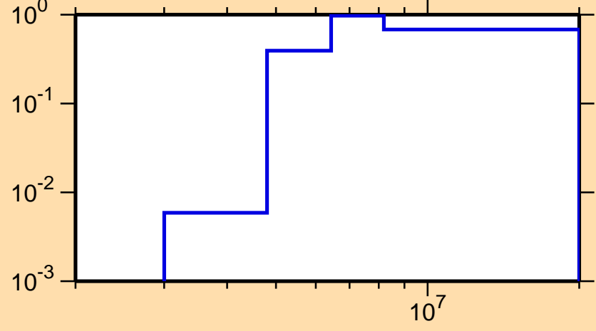
\sigma vs. E for ^{54}\text{Cr}(n,n\text{cont.})
