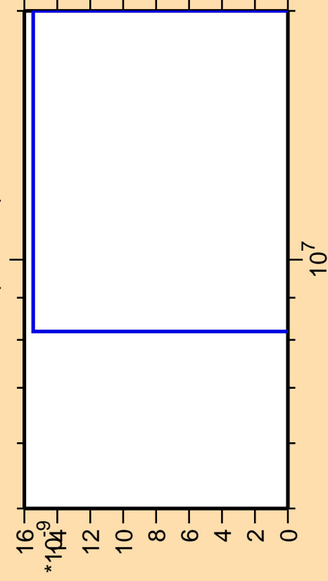
\Delta\sigma/\sigma vs. E for ^{54}\text{Cr}(\text{mt117})
