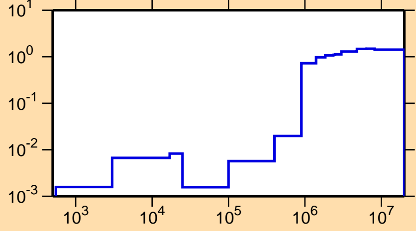
\sigma vs. E for ^{54}\text{Cr}(n,\text{nonel.})
