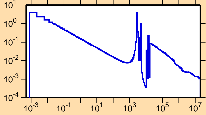
\sigma vs. E for ^{55}\text{Cr}(n,\gamma)
