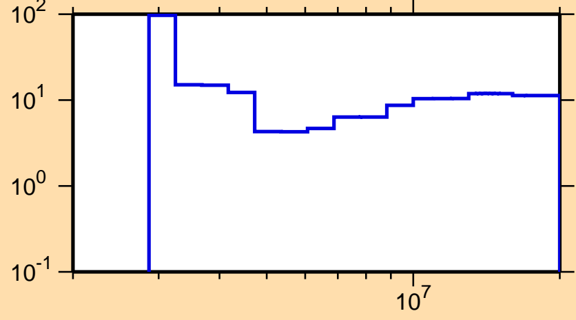
\Delta\sigma/\sigma vs. E for ^{55}\text{Cr}(n,ncont.)
