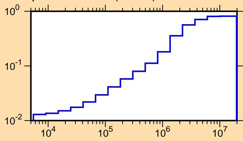
\mu vs. E for ^{55}\text{Cr}(\text{mt251})
