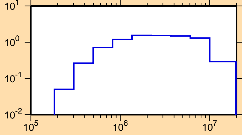
\sigma vs. E for ^{55}\text{Cr}(n,\text{inel.})
