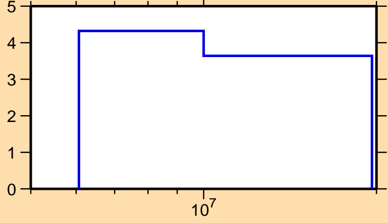
\Delta\sigma/\sigma vs. E for ^{55}\text{Cr}(n,2n)
