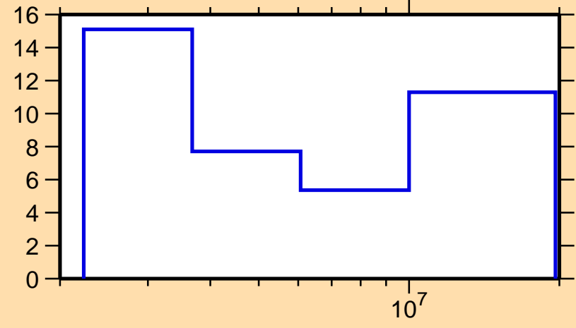
\Delta\sigma/\sigma vs. E for ^{55}\text{Cr}(n,n\text{cont.})
