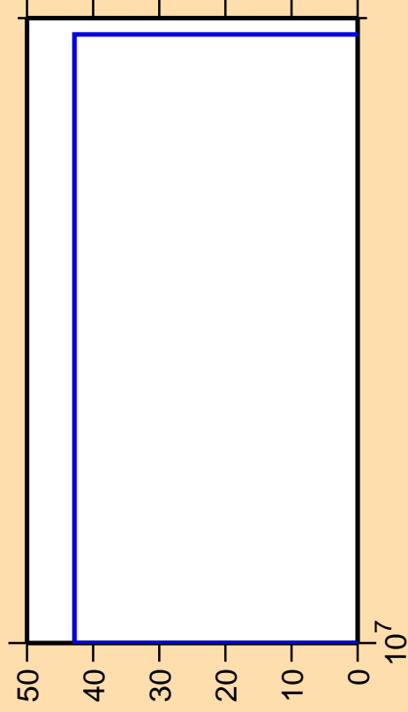
\Delta\sigma/\sigma vs. E for ^{55}\text{Cr}(n,nd)
