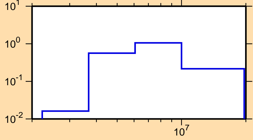
\sigma vs. E for ^{55}\text{Cr}(n,n\text{cont.})
