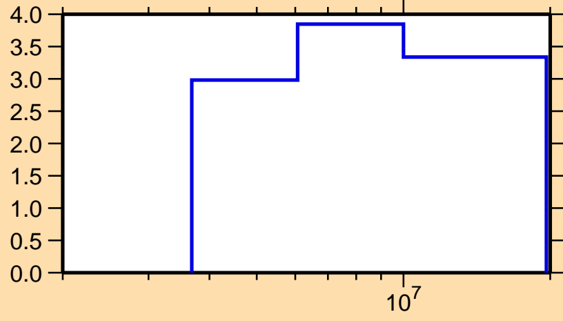
\Delta\sigma/\sigma vs. E for ^{55}\text{Cr}(n,el.)
