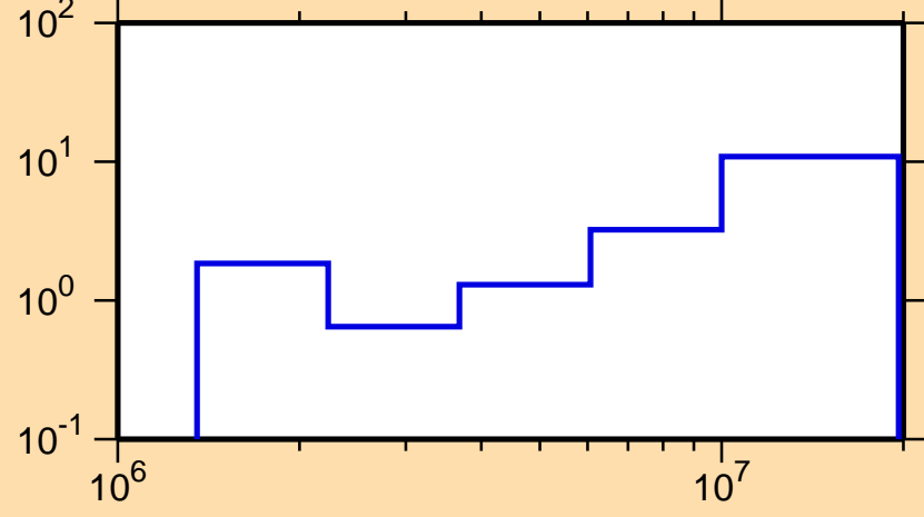
\Delta\sigma/\sigma vs. E for ^{55}\text{Cr}(n,\text{inel.})
