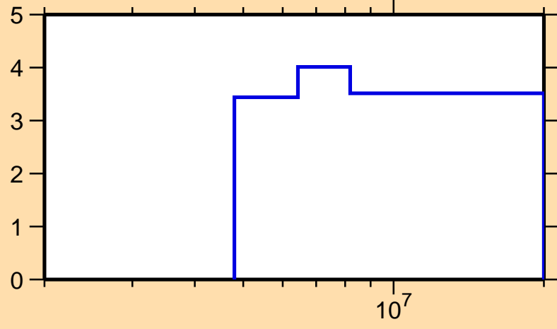
\Delta\sigma/\sigma vs. E for ^{55}\text{Cr}(n,el.)
