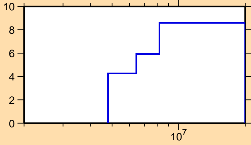
\Delta\sigma/\sigma vs. E for ^{55}\text{Cr}(n,ncont.)
