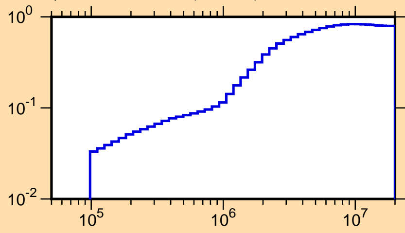
\mu vs. E for ^{56}\text{Cr}(\text{mt251})
