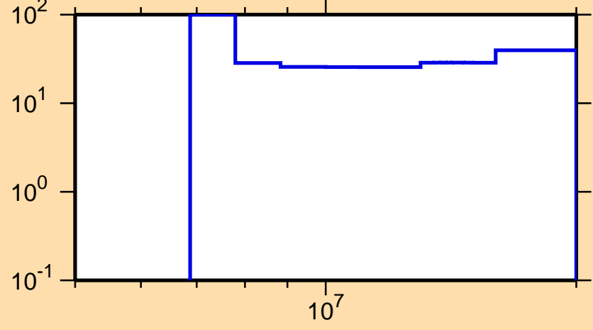
\Delta\sigma/\sigma vs. E for ^{58}\text{Cr}(n,2n)
