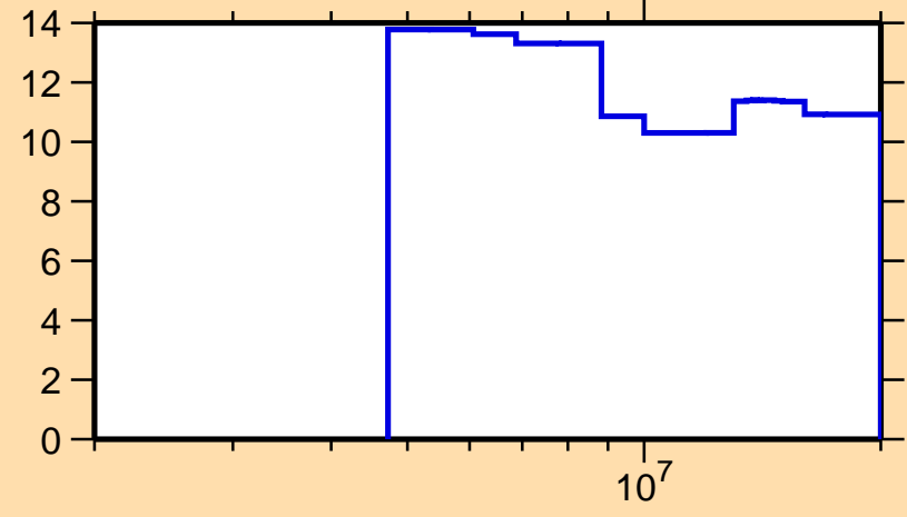
\Delta\sigma/\sigma vs. E for ^{58}\text{Cr}(n,n\text{onel.})
