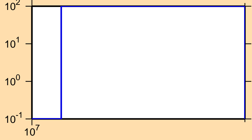
\Delta\sigma/\sigma vs. E for ^{58}\text{Cr}(n,p)
