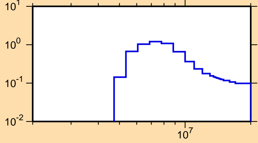
\sigma vs. E for ^{58}\text{Cr}(n,n\text{cont.})
