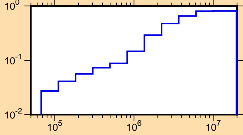
\mu vs. E for ^{58}\text{Cr}(\text{mt251})
