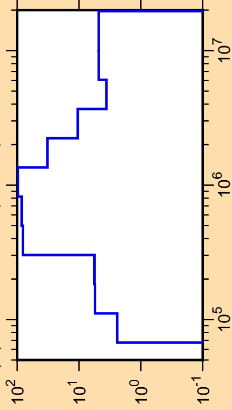
\Delta\mu/\mu vs. E for ^{58}\text{Cr}(\text{mt251})
