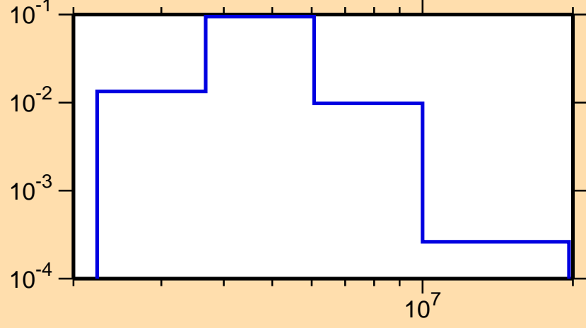
\sigma vs. E for ^{58}\text{Cr}(n,n_3)
