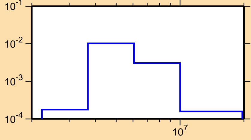
\sigma vs. E for ^{58}\text{Cr}(n,n_4)
