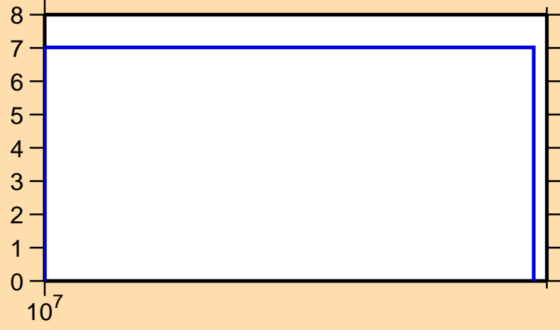
\Delta\sigma/\sigma vs. E for ^{58}\text{Cr}(n,\text{tot.})
