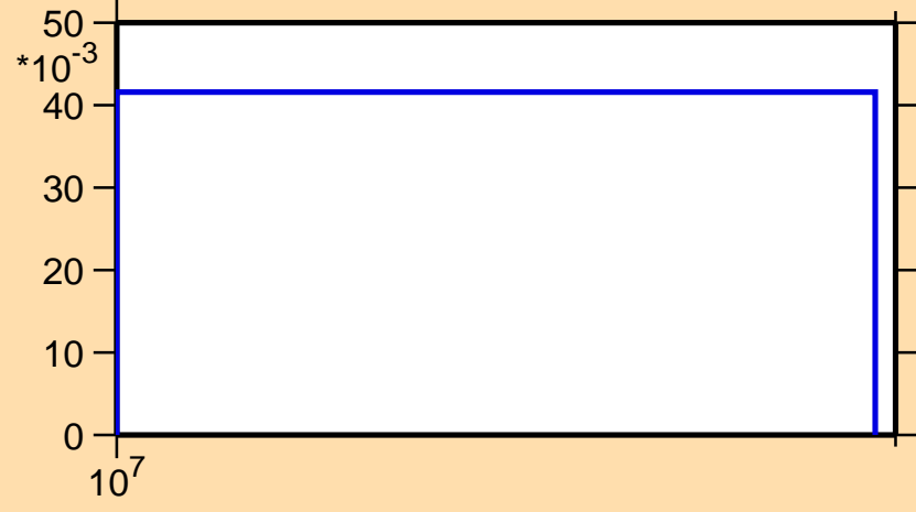
\sigma vs. E for ^{58}\text{Cr}(n,3n)
