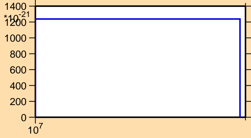
\sigma vs. E for ^{58}\text{Cr}(n,nd)
