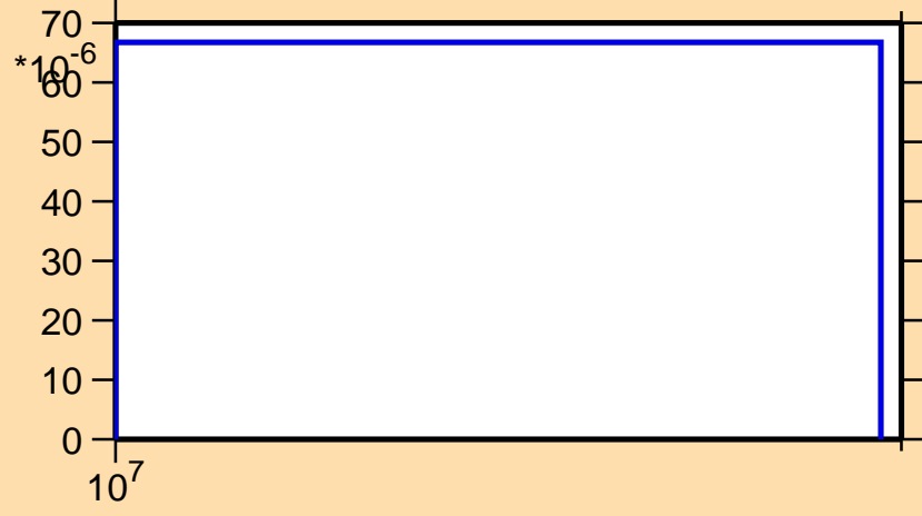
\sigma vs. E for ^{58}\text{Cr}(n,p)
