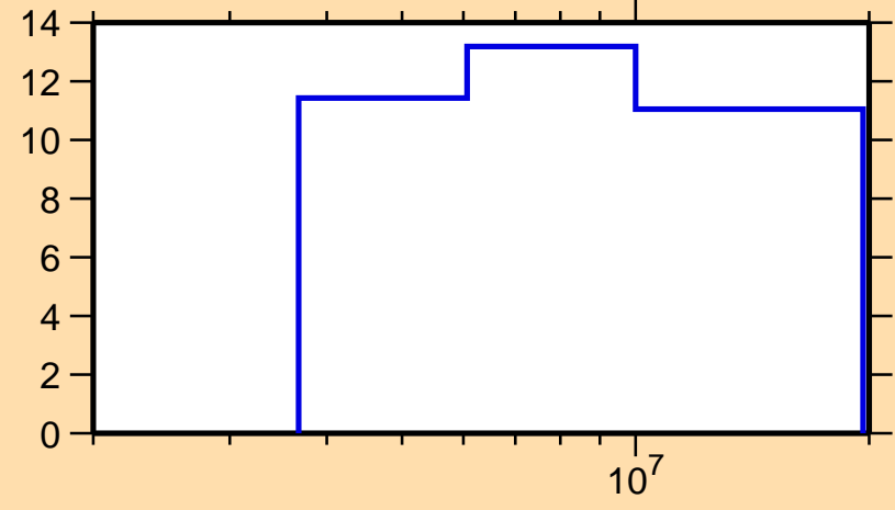
\Delta\sigma/\sigma vs. E for ^{58}\text{Cr}(n,n\text{onl.})
