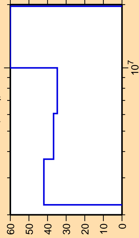
\Delta\sigma/\sigma vs. E for ^{58}\text{Cr}(n,n_4)
