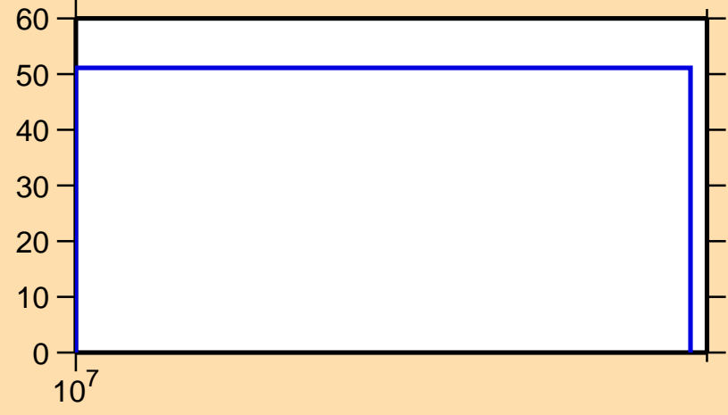
\Delta\sigma/\sigma vs. E for ^{58}\text{Cr}(n,ncont.)
