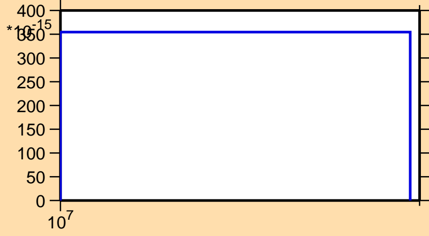
\sigma vs. E for ^{58}\text{Cr}(n,2n\alpha)
