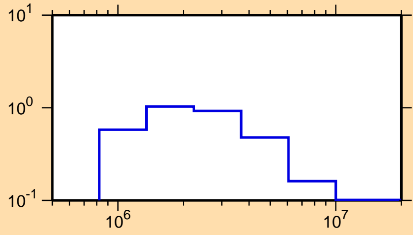
\sigma vs. E for ^{58}\text{Cr}(n,n_1)
