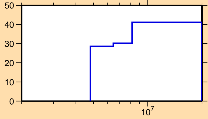
\Delta\sigma/\sigma vs. E for ^{58}\text{Cr}(n,n\text{cont.})
