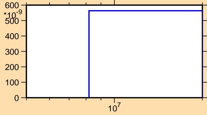
\sigma vs. E for ^{58}\text{Cr}(n,np)
