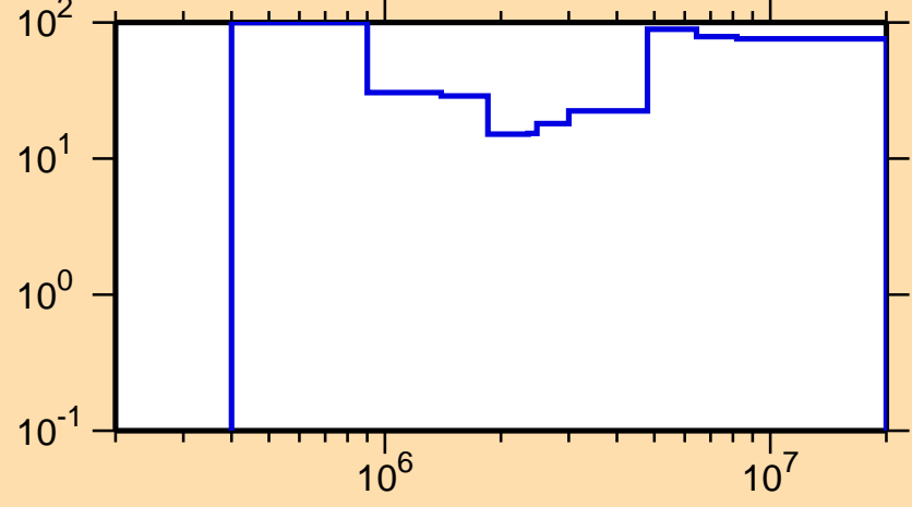
\Delta\sigma/\sigma vs. E for ^{58}\text{Cr}(n,n_1)
