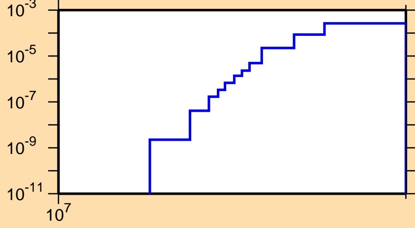
\sigma vs. E for ^{59}\text{Cr}(n,n\alpha)
