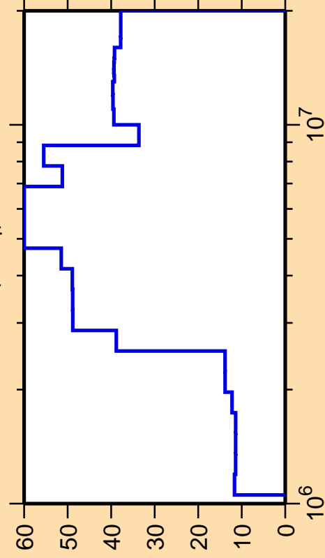
\Delta\sigma/\sigma vs. E for ^{59}\text{Cr}(n,n_4)
