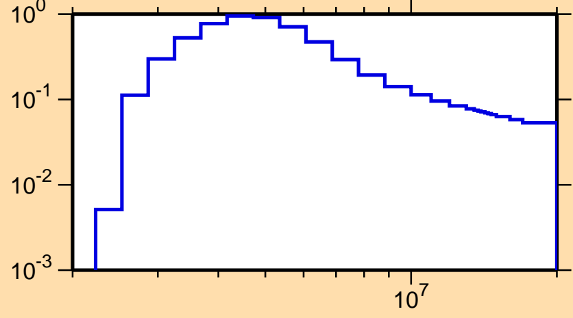
\sigma vs. E for ^{59}\text{Cr}(n,n\text{cont.})
