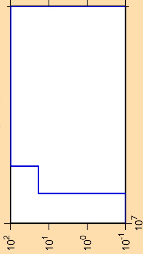
\Delta\sigma/\sigma vs. E for ^{59}\text{Cr}(n,n\alpha)
