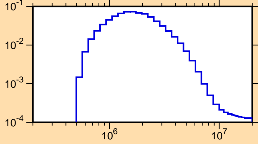
\sigma vs. E for ^{59}\text{Cr}(n,n_3)
