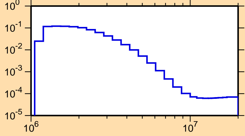
\sigma vs. E for ^{59}\text{Cr}(n,n_4)
