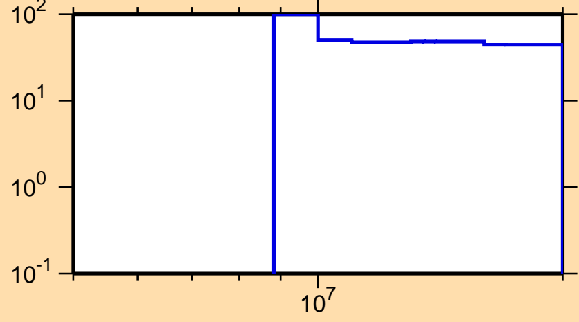
\Delta\sigma/\sigma vs. E for ^{59}\text{Cr}(n,p)
