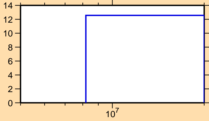
\Delta\sigma/\sigma vs. E for ^{59}\text{Cr}(n,el.)
