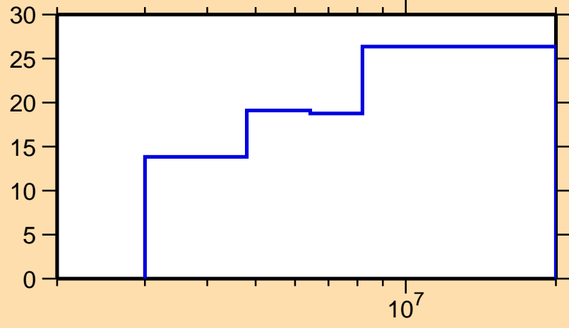
\Delta\sigma/\sigma vs. E for ^{59}\text{Cr}(n,\text{inel.})
