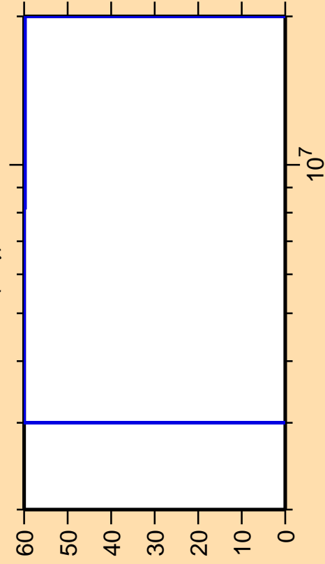
\Delta\sigma/\sigma vs. E for ^{59}\text{Cr}(n,\gamma)
