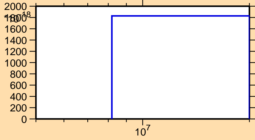
\sigma vs. E for ^{59}\text{Cr}(n,2np)
