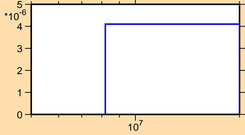
\sigma vs. E for ^{59}\text{Cr}(n,d)
