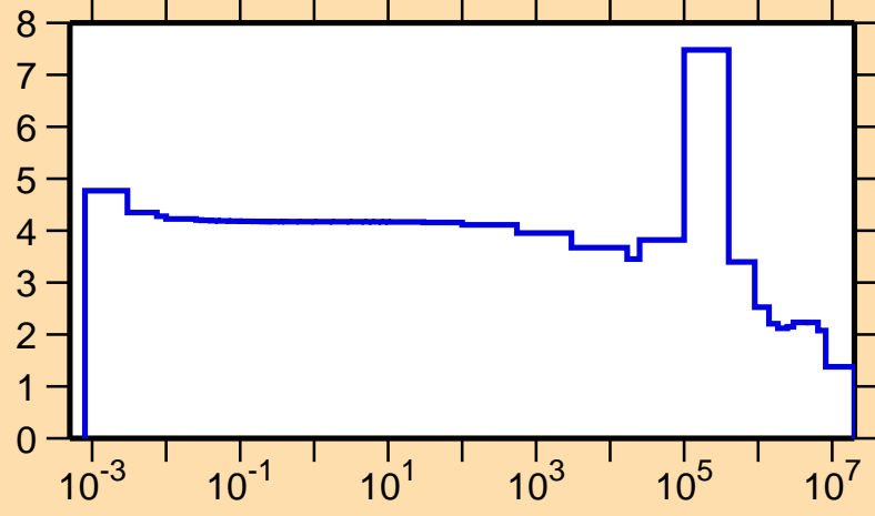
\sigma vs. E for ^{59}\text{Cr}(n,\text{el.})
