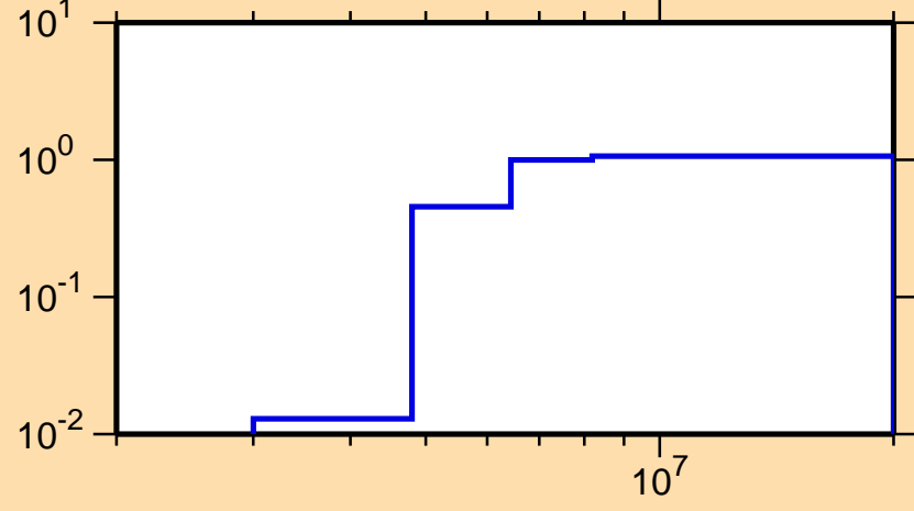
\sigma vs. E for ^{59}\text{Cr}(n,2n)
