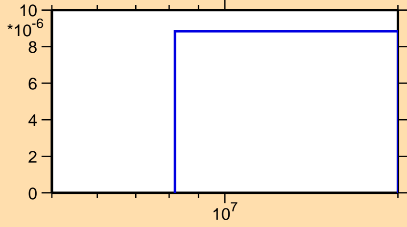
\sigma vs. E for ^{59}\text{Cr}(n,\alpha)
