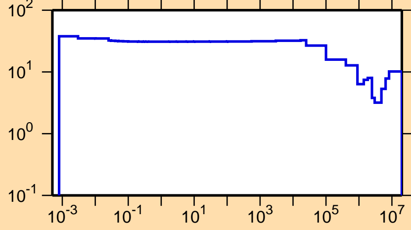
\Delta\sigma/\sigma vs. E for ^{59}\text{Cr}(n,\text{tot.})
