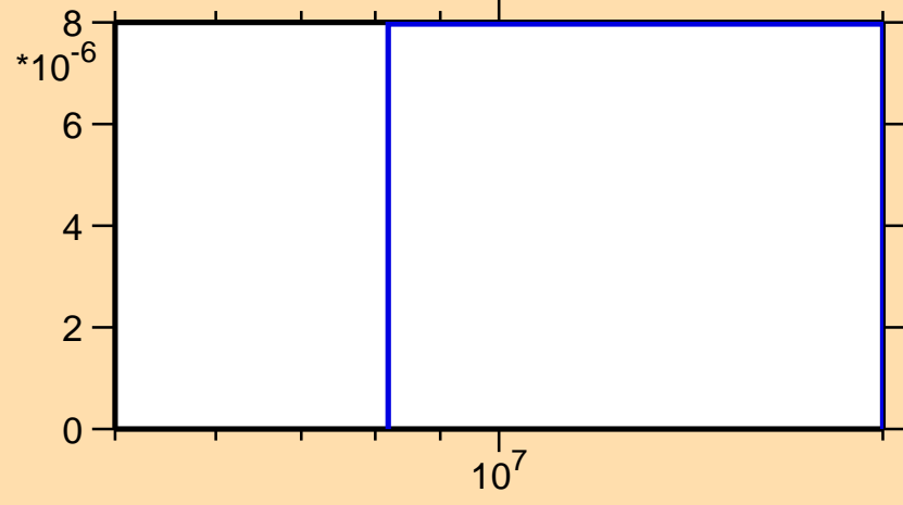
\sigma vs. E for ^{59}\text{Cr}(n,t)
