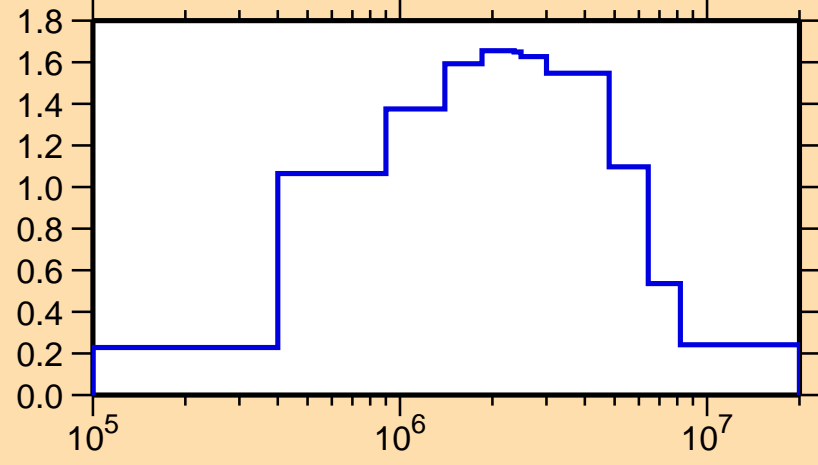
\sigma vs. E for ^{59}\text{Cr}(n,\text{inel.})
