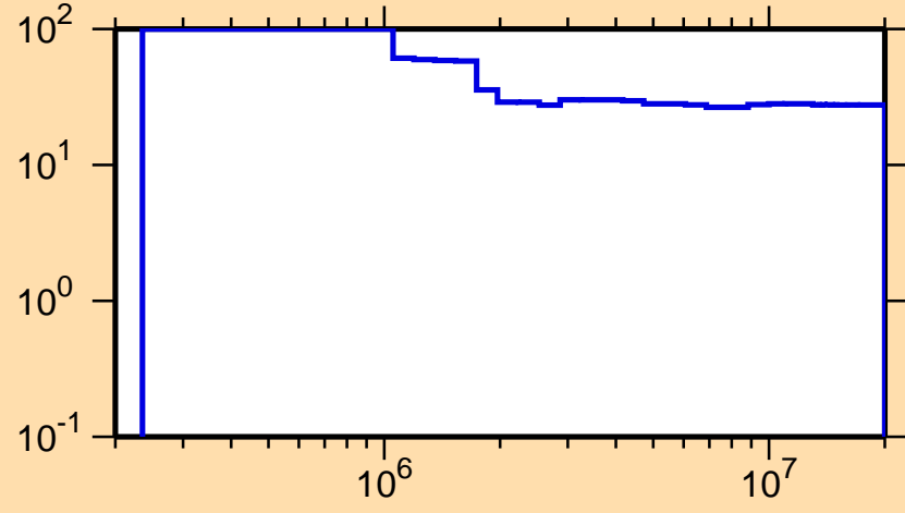
\Delta\sigma/\sigma vs. E for ^{115}\text{Cs}(n,inel.)
