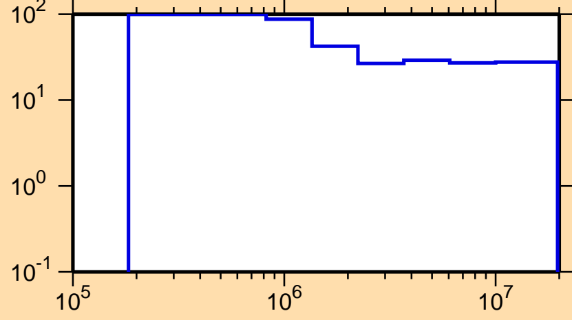
\Delta\sigma/\sigma vs. E for ^{115}\text{Cs}(n,\text{inel.})
