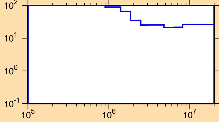
\Delta\sigma/\sigma vs. E for ^{115}\text{Cs}(n,n_1)
