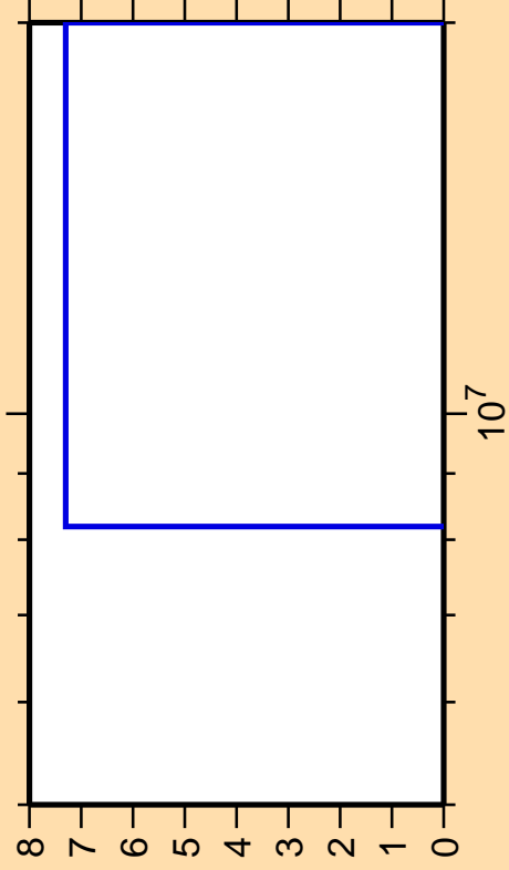
\Delta\sigma/\sigma vs. E for ^{115}\text{Cs}(n,2n\alpha)
