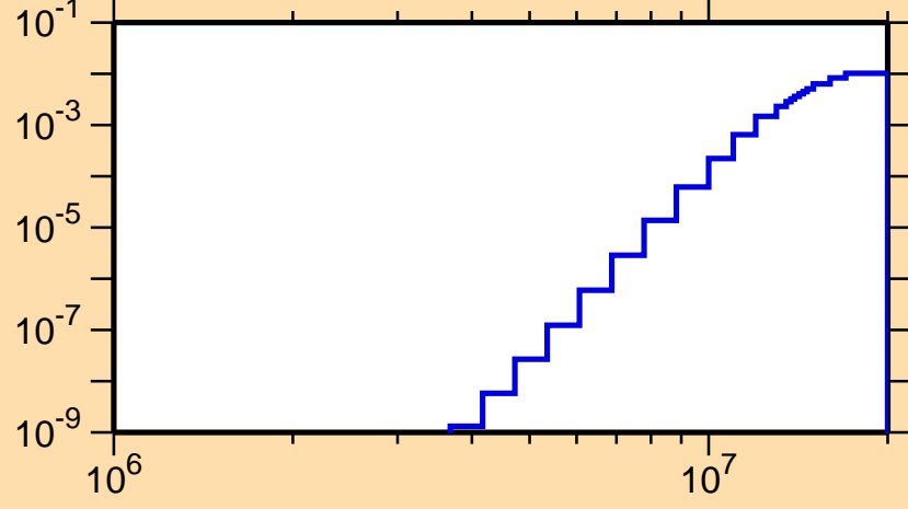
\sigma vs. E for ^{116}\text{Cs}(n,\text{He3})
