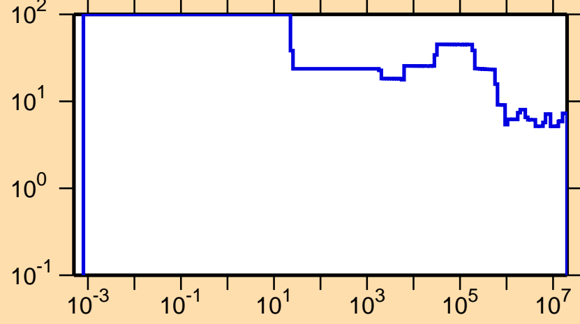
\Delta\sigma/\sigma vs. E for ^{116}\text{Cs}(n,\text{tot.})
