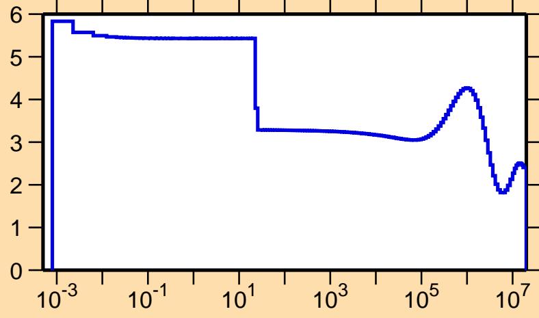
\sigma vs. E for ^{116}\text{Cs}(n,\text{el.})
