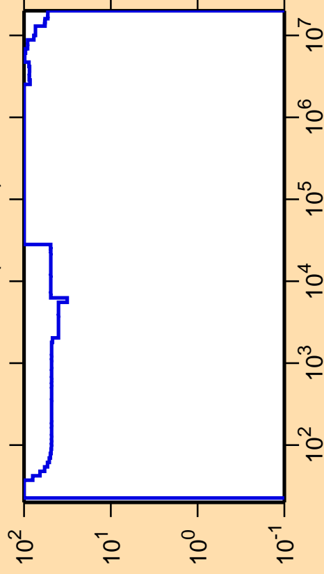
\Delta\sigma/\sigma vs. E for ^{116}\text{Cs}(n,\text{inel.})
