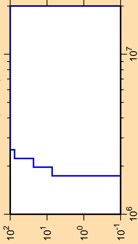
\Delta\sigma/\sigma vs. E for ^{116}\text{Cs}(n,\text{He3})
