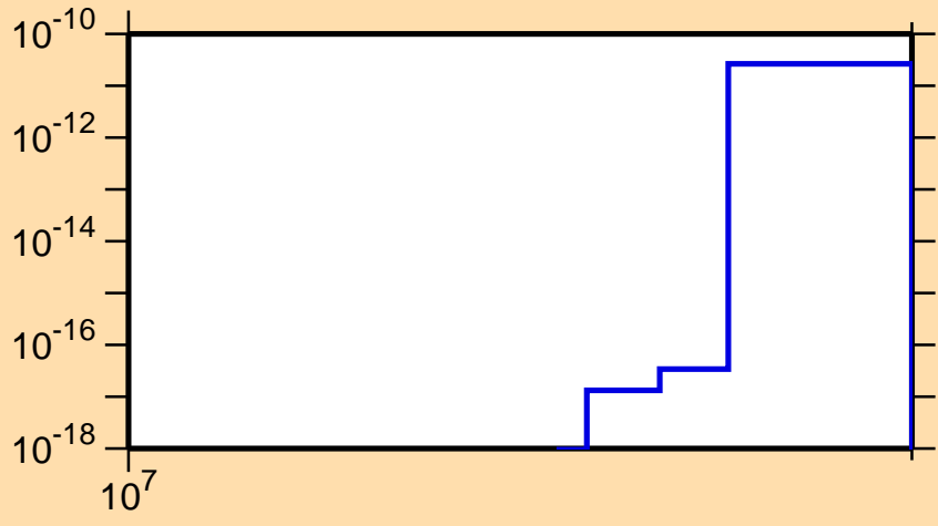
\sigma vs. E for ^{116}\text{Cs}(n,nt)
