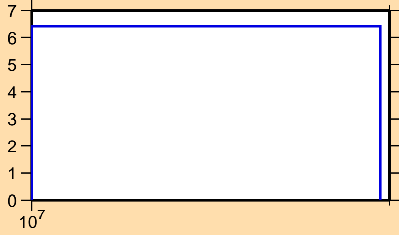
\Delta\sigma/\sigma vs. E for ^{116}\text{Cs}(n,\text{nonel.})
