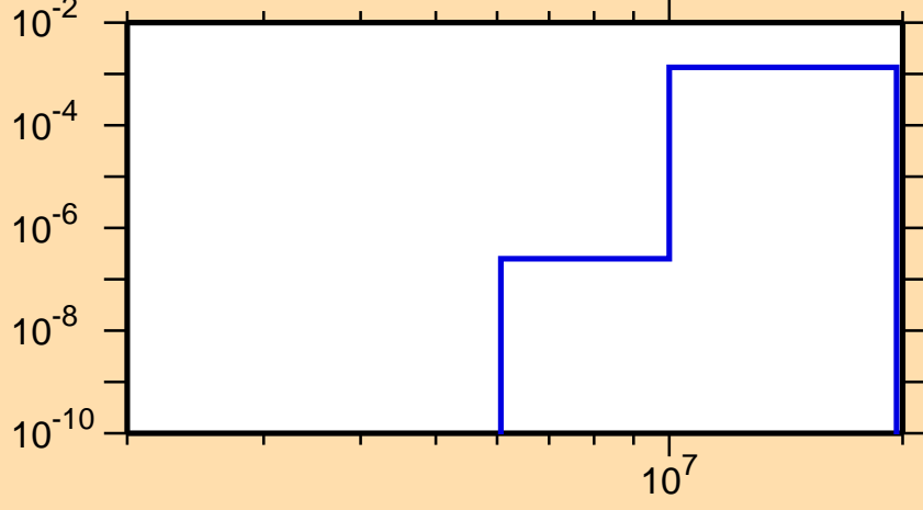
\sigma vs. E for ^{116}\text{Cs}(\text{mt } 45)
