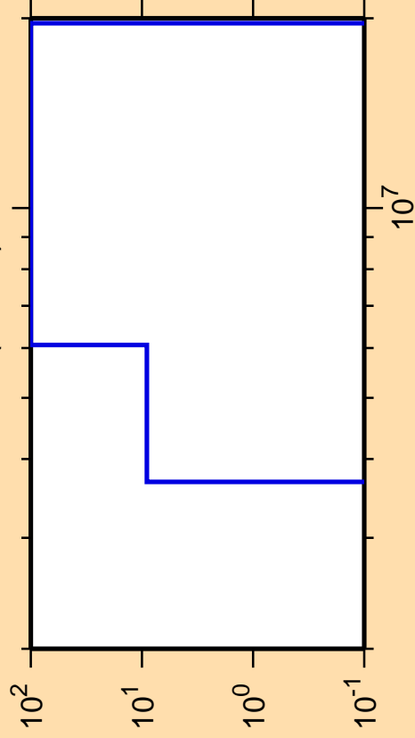
\Delta\sigma/\sigma vs. E for ^{116}\text{Cs}(\text{mt } 45)
