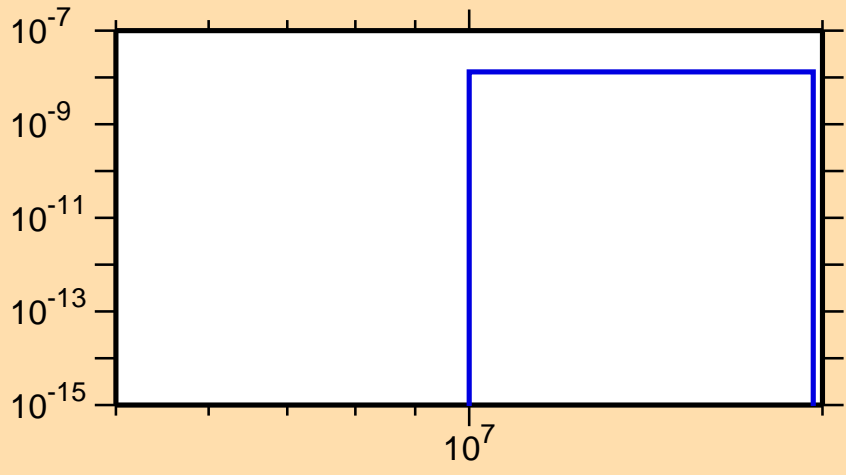
\sigma vs. E for ^{116}\text{Cs} (mt 34)
