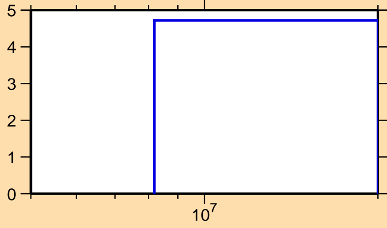
\Delta\sigma/\sigma vs. E for ^{116}\text{Cs}(n,\text{el.})
