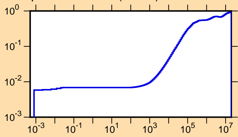
\mu vs. E for ^{117}\text{Cs}(\text{mt251})
