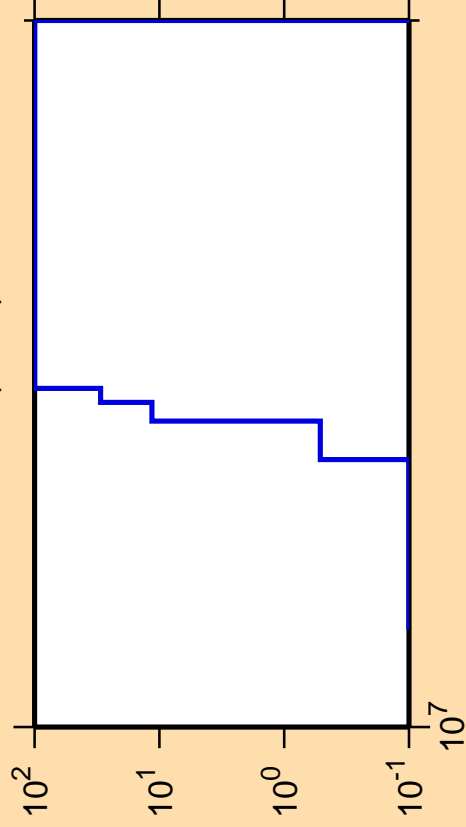
\Delta\sigma/\sigma vs. E for ^{117}\text{Cs}(n,nd)
