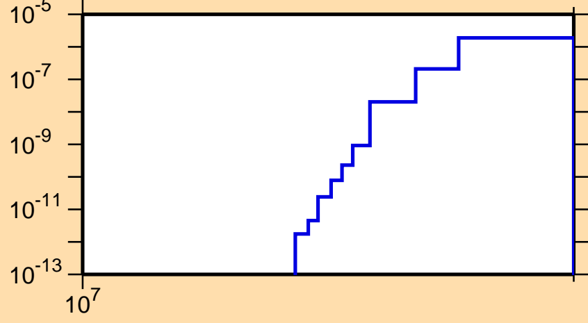
\sigma vs. E for ^{117}\text{Cs}(n,nd)
