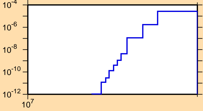
\sigma vs. E for ^{117}\text{Cs}(n,pt)
