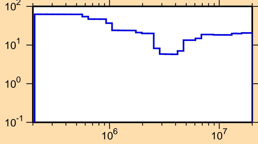
\Delta\sigma/\sigma vs. E for ^{117}\text{Cs}(n,\text{nonel.})
