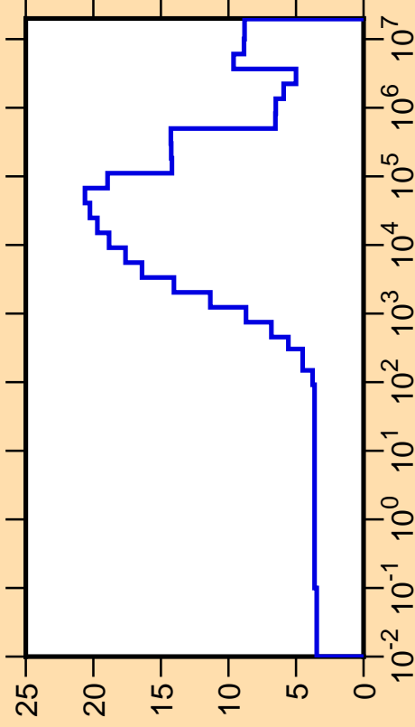
\Delta\mu/\mu vs. E for ^{118}\text{Cs}(\text{mt251})
