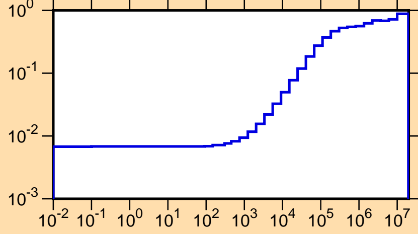
\mu vs. E for ^{118}\text{Cs}(\text{mt251})
