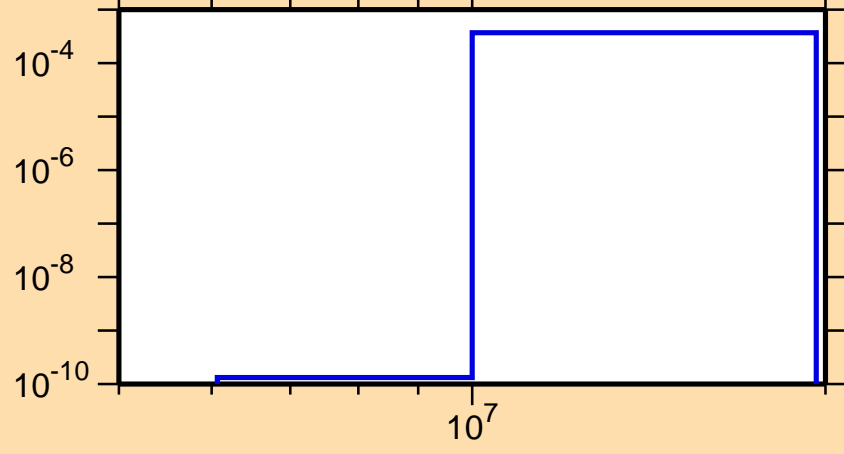
\sigma vs. E for ^{118}\text{Cs}(n,\text{pd})
