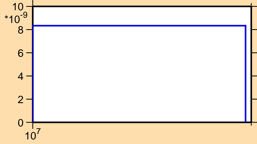
\sigma vs. E for ^{118}\text{Cs} (mt 34)
