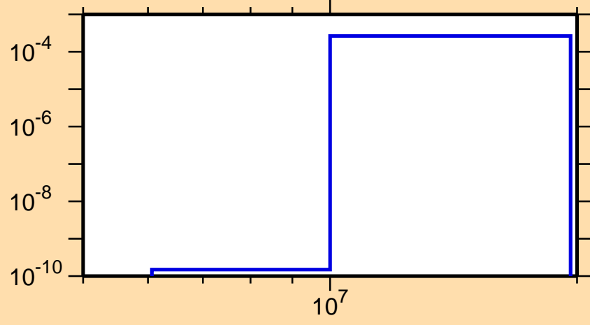
\sigma vs. E for ^{118}\text{Cs}(\text{mt } 45)
