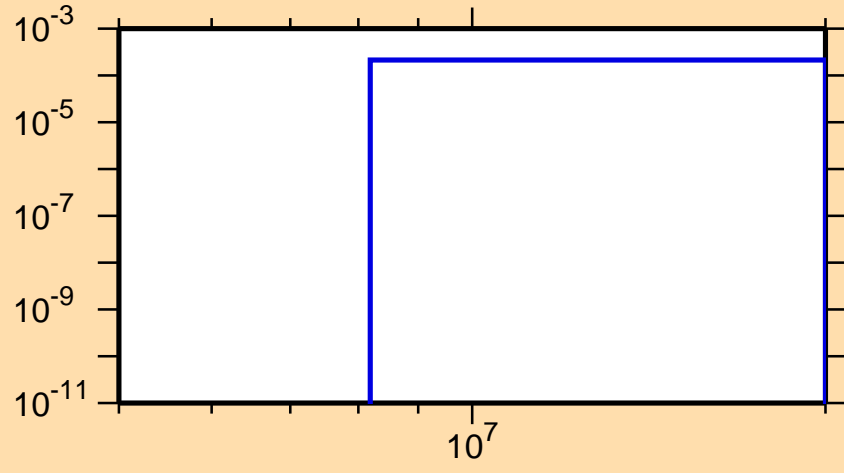
\sigma vs. E for ^{118}\text{Cs}(\text{mt } 45)
