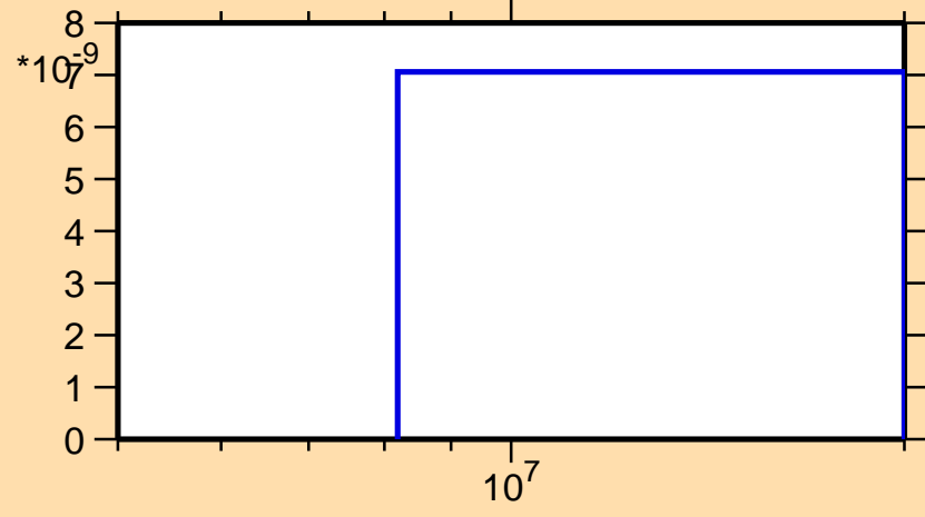
\sigma vs. E for ^{118}\text{Cs}(\text{mt } 34)
