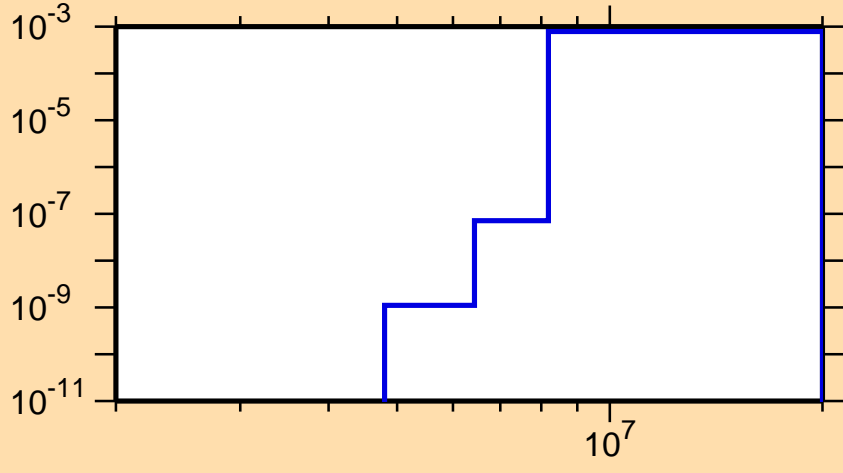
\sigma vs. E for ^{118}\text{Cs}(n,\text{He}3)
