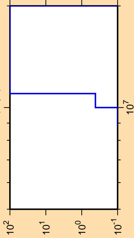
\Delta\sigma/\sigma vs. E for ^{118}\text{Cs}(n,pt)
