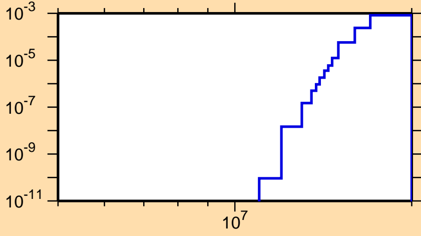
\sigma vs. E for ^{118}\text{Cs}(n,pt)
