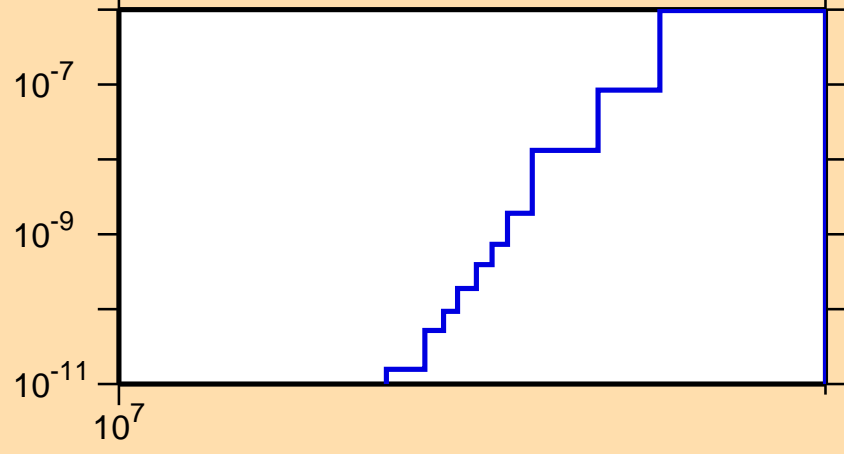
\sigma vs. E for ^{118}\text{Cs} (mt 34)
