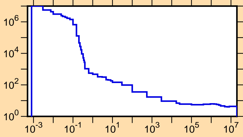
\sigma vs. E for ^{118}\text{Cs}(n,\text{tot.})
