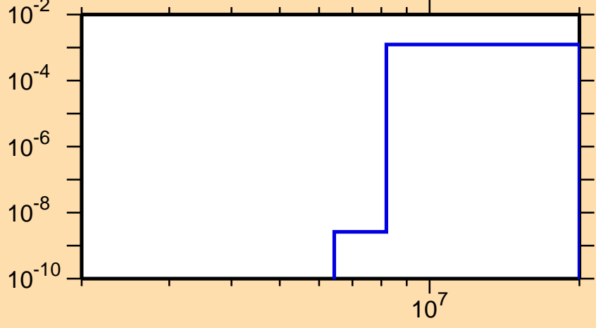
\sigma vs. E for ^{118}\text{Cs}(n,t)
