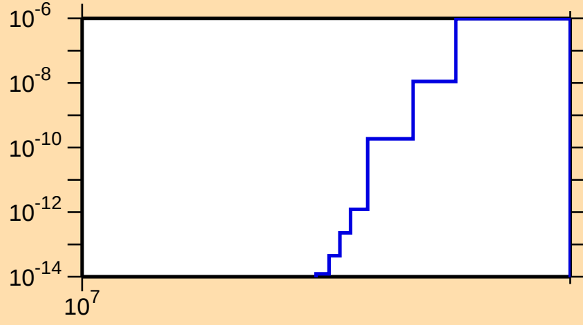
\sigma vs. E for ^{119}\text{Cs}(n,\text{pt})
