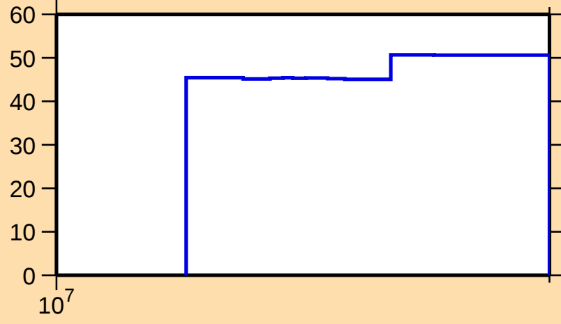
\Delta\sigma/\sigma vs. E for ^{119}\text{Cs}(n,\text{el.})
