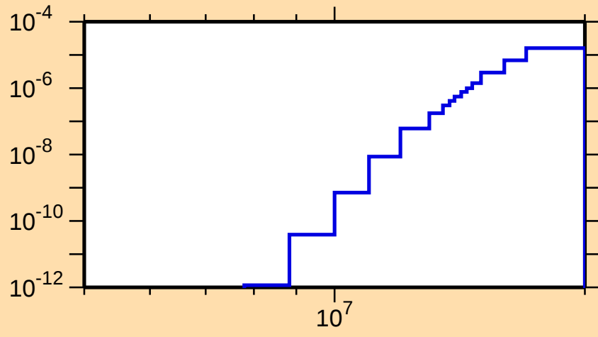
\sigma vs. E for ^{119}\text{Cs}(\text{mt117})
