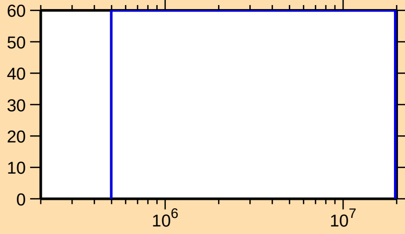
\Delta\sigma/\sigma vs. E for ^{119}\text{Cs}(n,ncont.)
