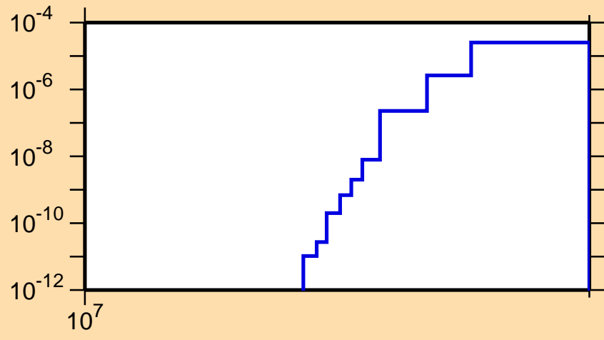
\sigma vs. E for ^{119}\text{Cs}(n,nd)
