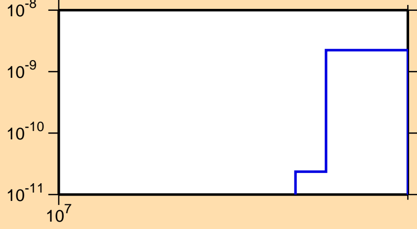
\sigma vs. E for ^{119}\text{Cs} (mt 34)
