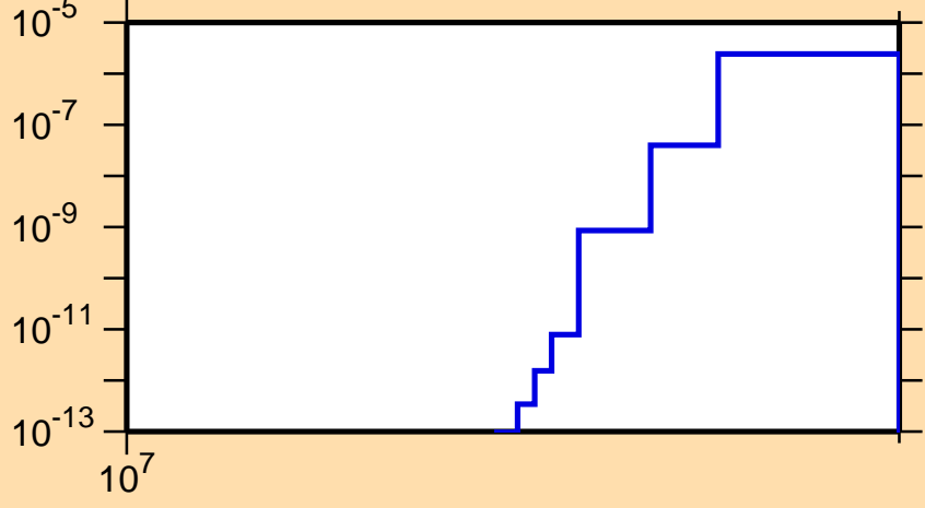
\sigma vs. E for ^{119}\text{Cs}(n,pt)
