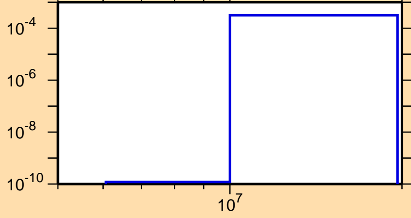
\sigma vs. E for ^{119}\text{Cs}(n,t)
