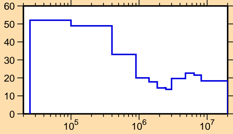
\Delta\sigma/\sigma vs. E for ^{119}\text{Cs}(n,nonel.)
