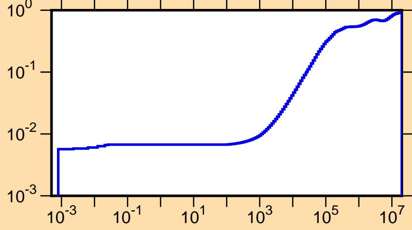
\mu vs. E for ^{120}\text{Cs}(\text{mt251})
