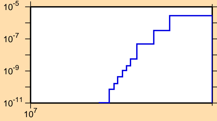
\sigma vs. E for ^{120}\text{Cs}(n,2n\alpha)
