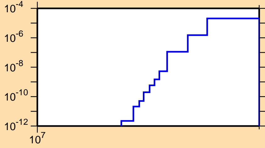
\sigma vs. E for ^{120}\text{Cs}(n,pt)
